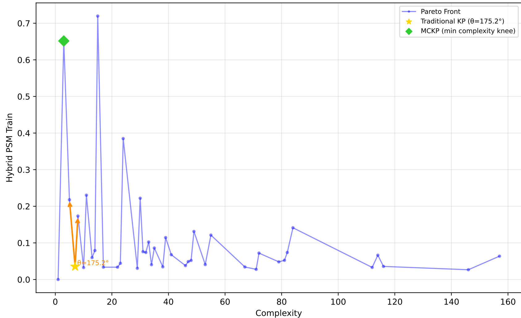
678_visualizing_environmental - Run 29 - SVP - Hybrid PSM Train \lambda_1=0.40, \lambda_2=0.00, \lambda_3=0.00 | Difficulty: 0.53 | Method: mckp
