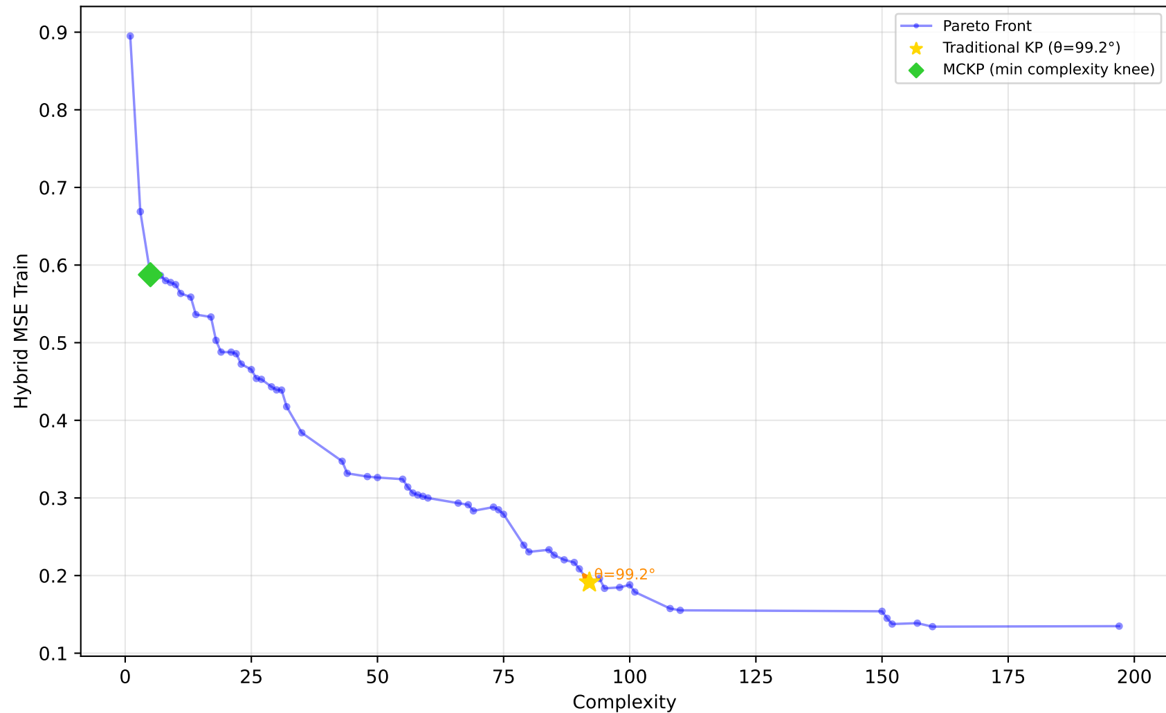
678_visualizing_environmental - Run 2 - MVP - Hybrid MSE Train \lambda_1=0.00, \lambda_2=0.00, \lambda_3=0.10 | Difficulty: 0.19 | Method: mckp
