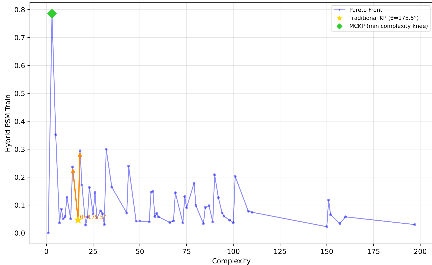
678_visualizing_environmental - Run 2 - MVP - Hybrid PSM Train \lambda_1=0.40, \lambda_2=0.00, \lambda_3=0.00 | Difficulty: 0.19 | Method: mckp
