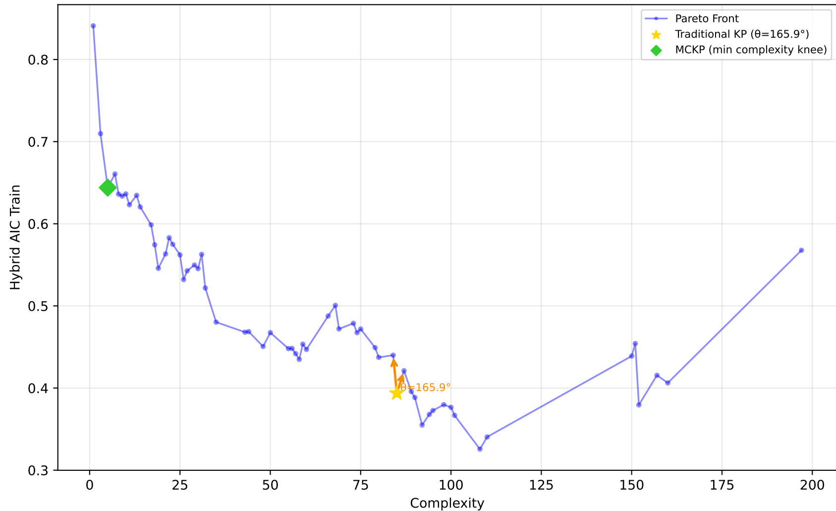
678_visualizing_environmental - Run 2 - SVP - Hybrid AIC Train \lambda_1=0.40, \lambda_2=0.00, \lambda_3=0.00 | Difficulty: 0.19 | Method: mckp
