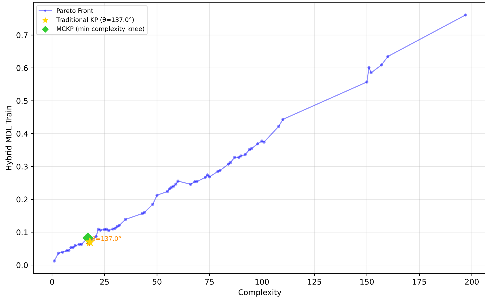
678_visualizing_environmental - Run 2 - SVP - Hybrid MDL Train \lambda_1=0.40, \lambda_2=0.00, \lambda_3=0.00 | Difficulty: 0.19 | Method: mckp
