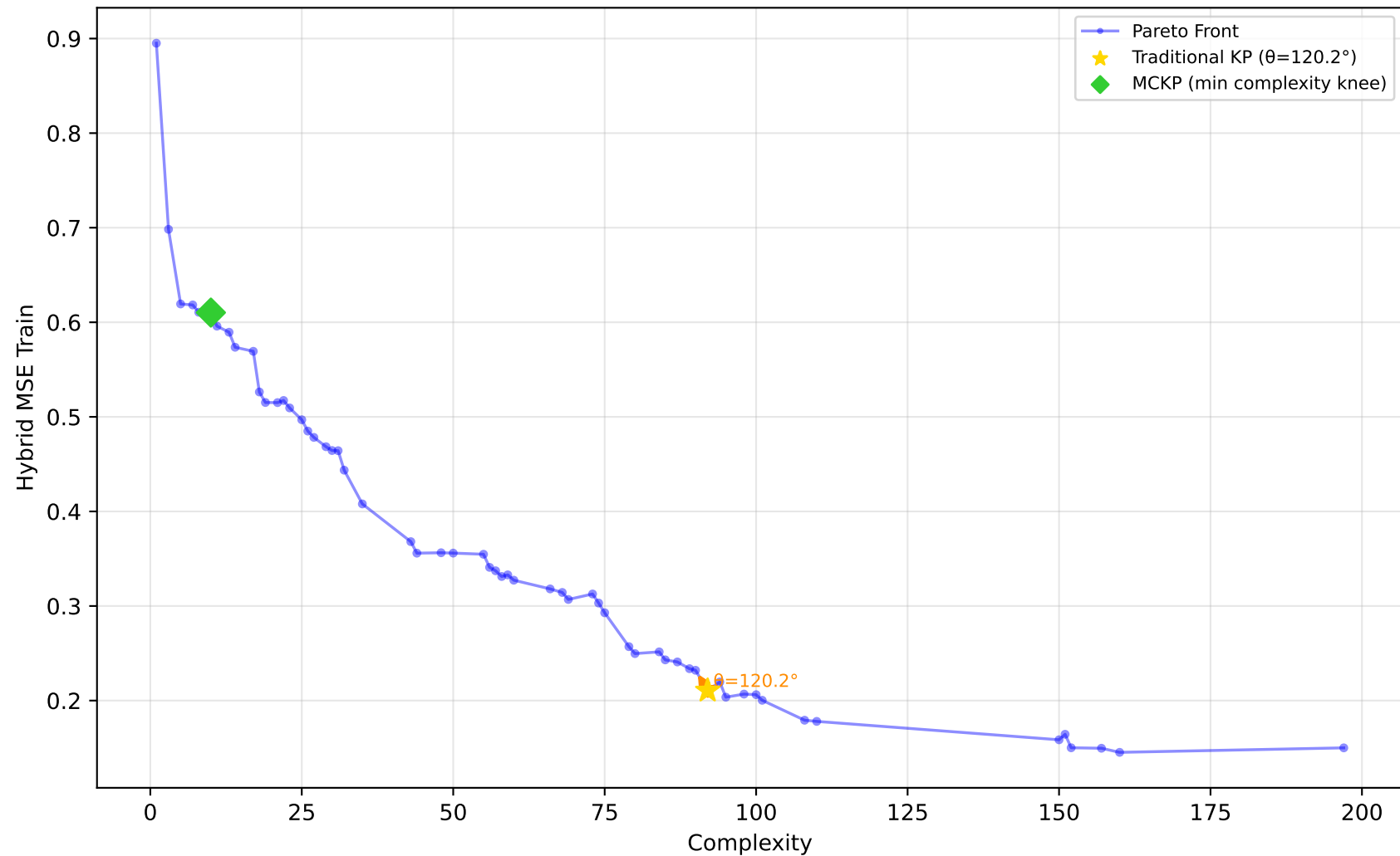
678_visualizing_environmental - Run 2 - SVP - Hybrid MSE Train \lambda_1=0.40, \lambda_2=0.00, \lambda_3=0.00 | Difficulty: 0.19 | Method: mckp
