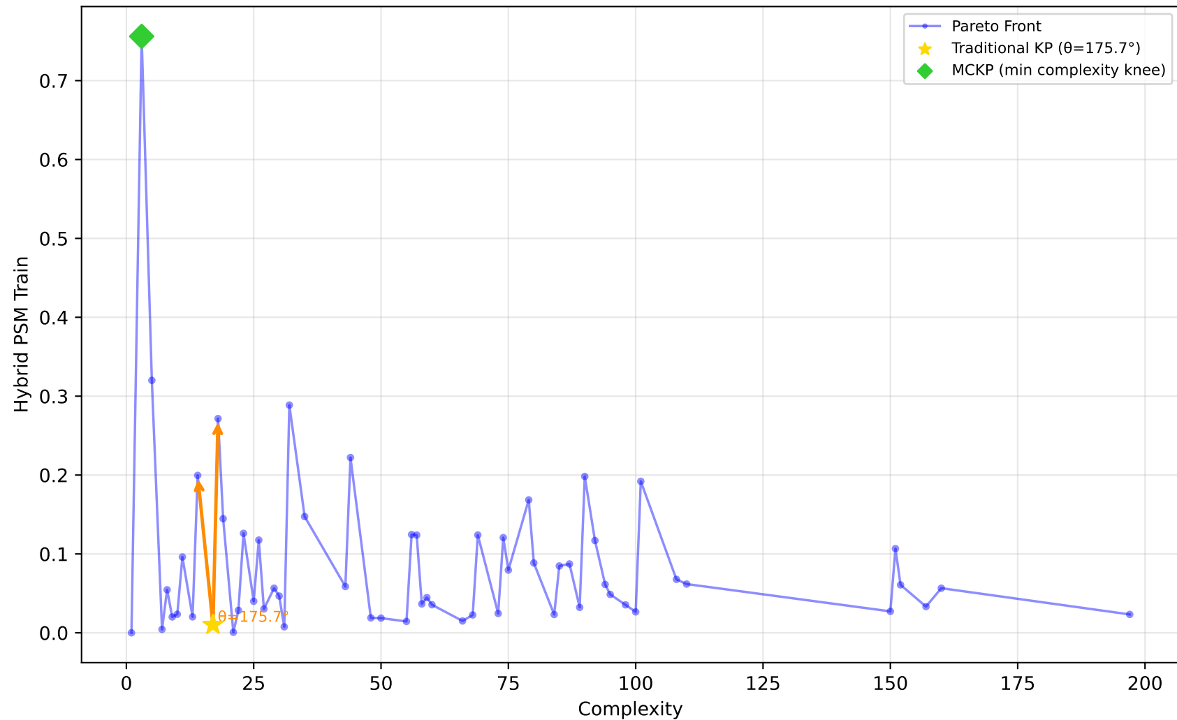
678_visualizing_environmental - Run 2 - SVP - Hybrid PSM Train \lambda_1=0.00, \lambda_2=0.10, \lambda_3=0.20 | Difficulty: 0.19 | Method: mckp
