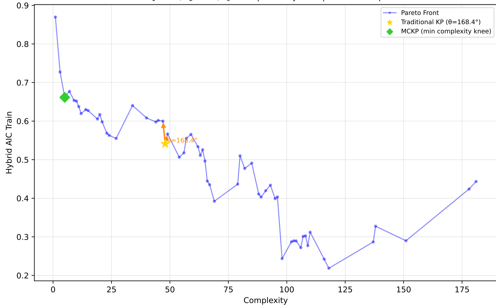
678_visualizing_environmental - Run 30 - MVP - Hybrid AIC Train \lambda_1=0.00 , \lambda_2=0.00 , \lambda_3=0.10 | Difficulty: 0.38 | Method: mckp
