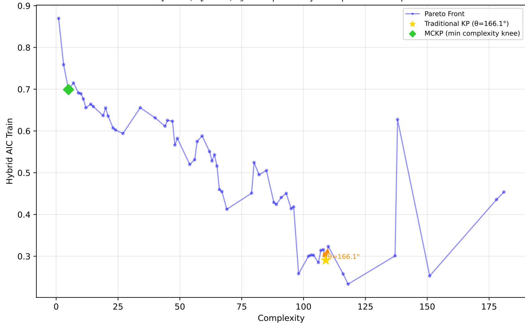
678_visualizing_environmental - Run 30 - MVP - Hybrid AIC Train \lambda_1=0.40, \lambda_2=0.00, \lambda_3=0.00 | Difficulty: 0.38 | Method: mckp
