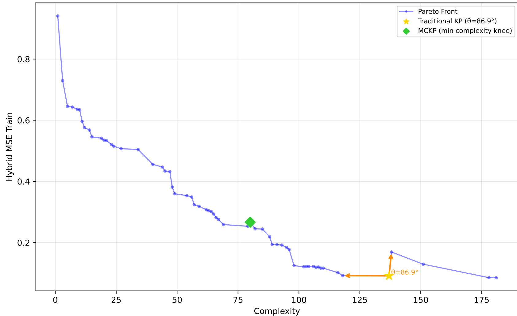
678_visualizing_environmental - Run 30 - MVP - Hybrid MSE Train \lambda_1=0.00, \lambda_2=0.00, \lambda_3=0.10 | Difficulty: 0.38 | Method: mckp
