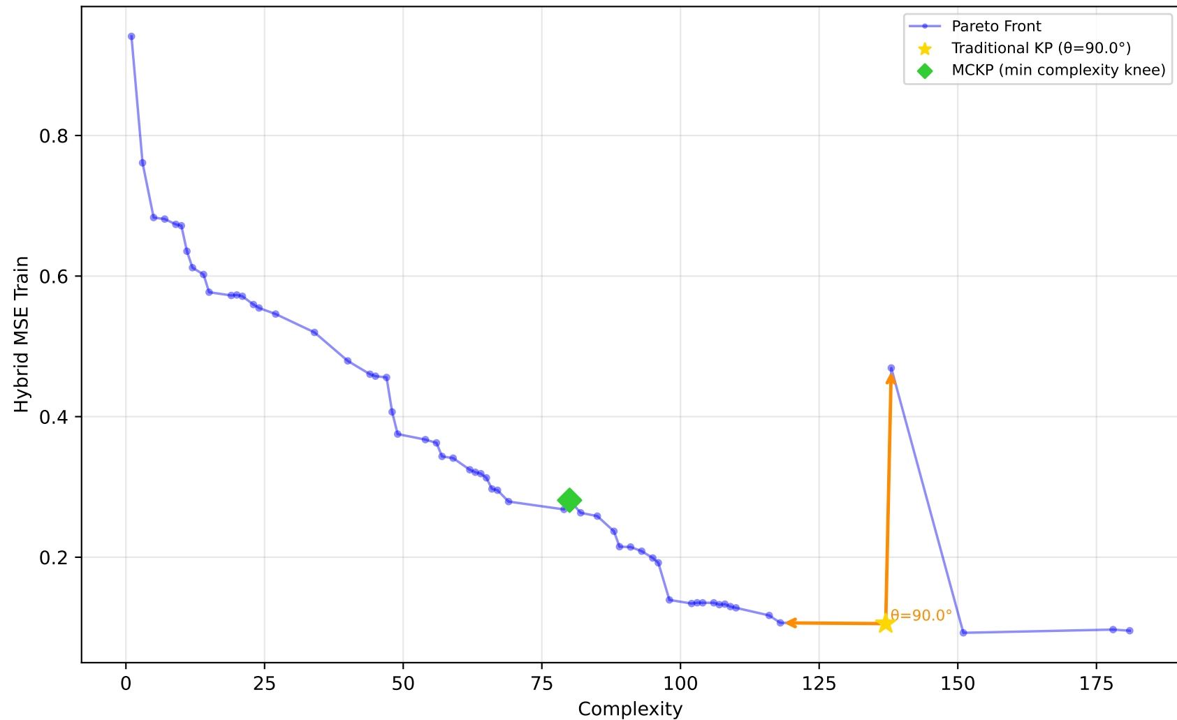
678_visualizing_environmental - Run 30 - MVP - Hybrid MSE Train \lambda_1=0.40 , \lambda_2=0.00 , \lambda_3=0.00 | Difficulty: 0.38 | Method: mckp
