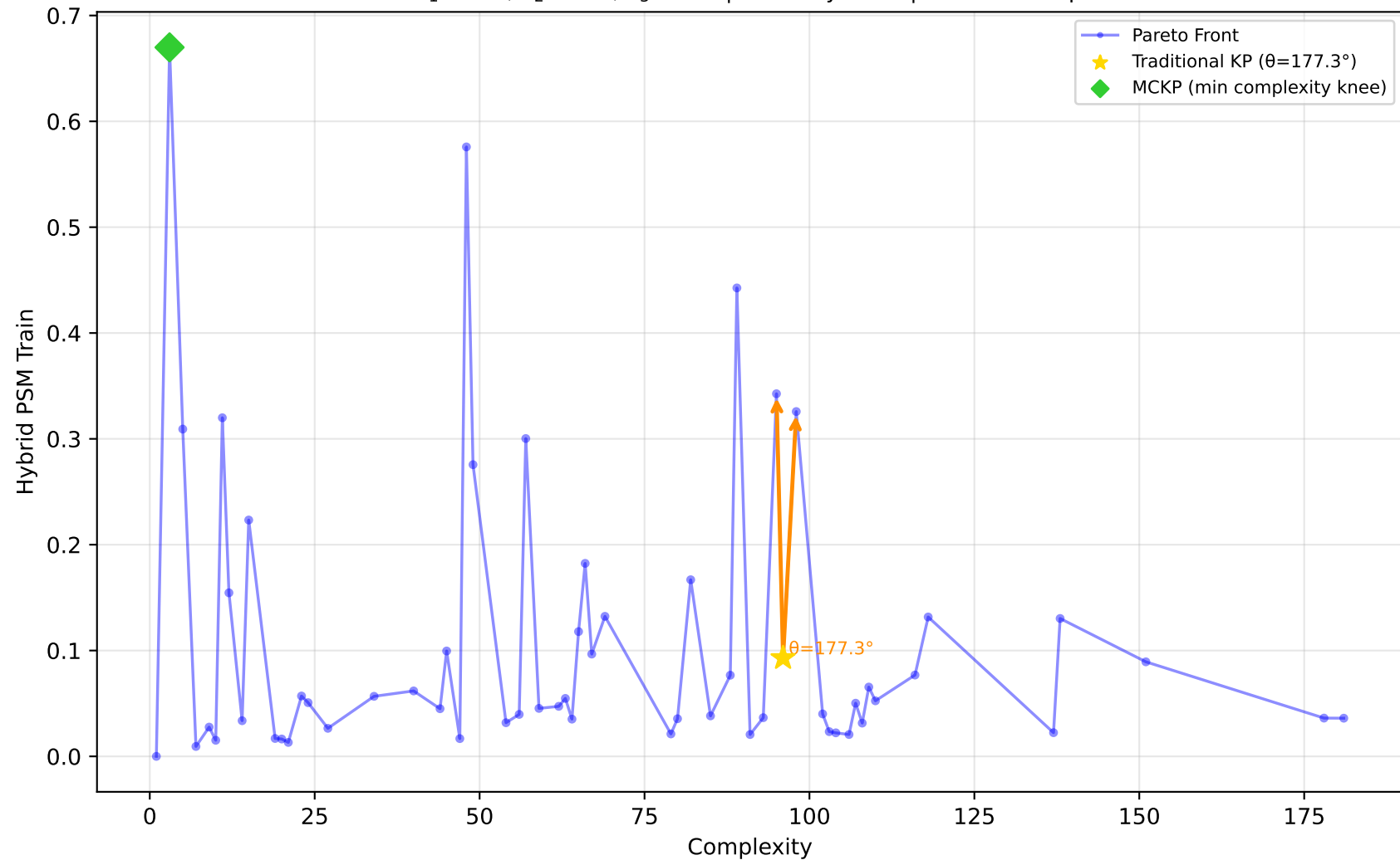
678_visualizing_environmental - Run 30 - MVP - Hybrid PSM Train \lambda_1=0.00, \lambda_2=0.00, \lambda_3=0.10 | Difficulty: 0.38 | Method: mckp
