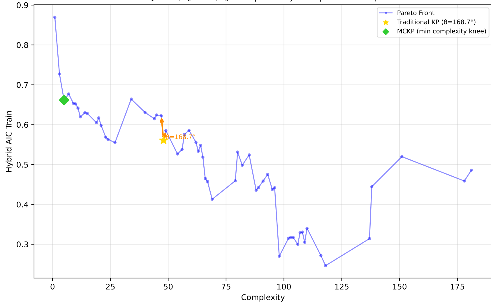
678_visualizing_environmental - Run 30 - SVP - Hybrid AIC Train \lambda_1=0.00, \lambda_2=0.10, \lambda_3=0.20 | Difficulty: 0.38 | Method: mckp
