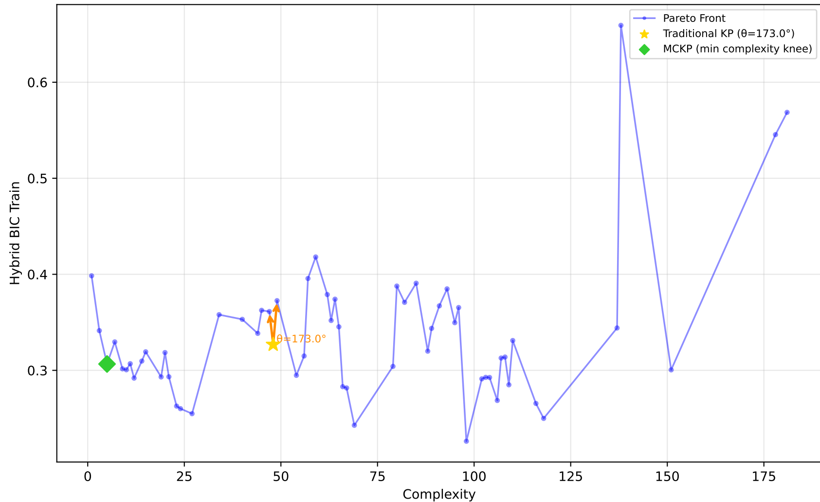
678_visualizing_environmental - Run 30 - SVP - Hybrid BIC Train \lambda_1=0.40, \lambda_2=0.00, \lambda_3=0.00 | Difficulty: 0.38 | Method: mckp
