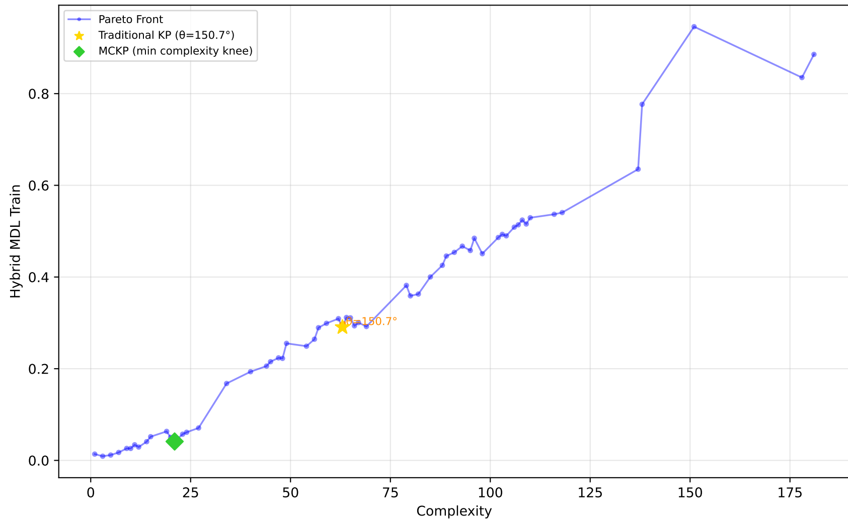
678_visualizing_environmental - Run 30 - SVP - Hybrid MDL Train \lambda_1=0.00, \lambda_2=0.10, \lambda_3=0.20 | Difficulty: 0.38 | Method: mckp
