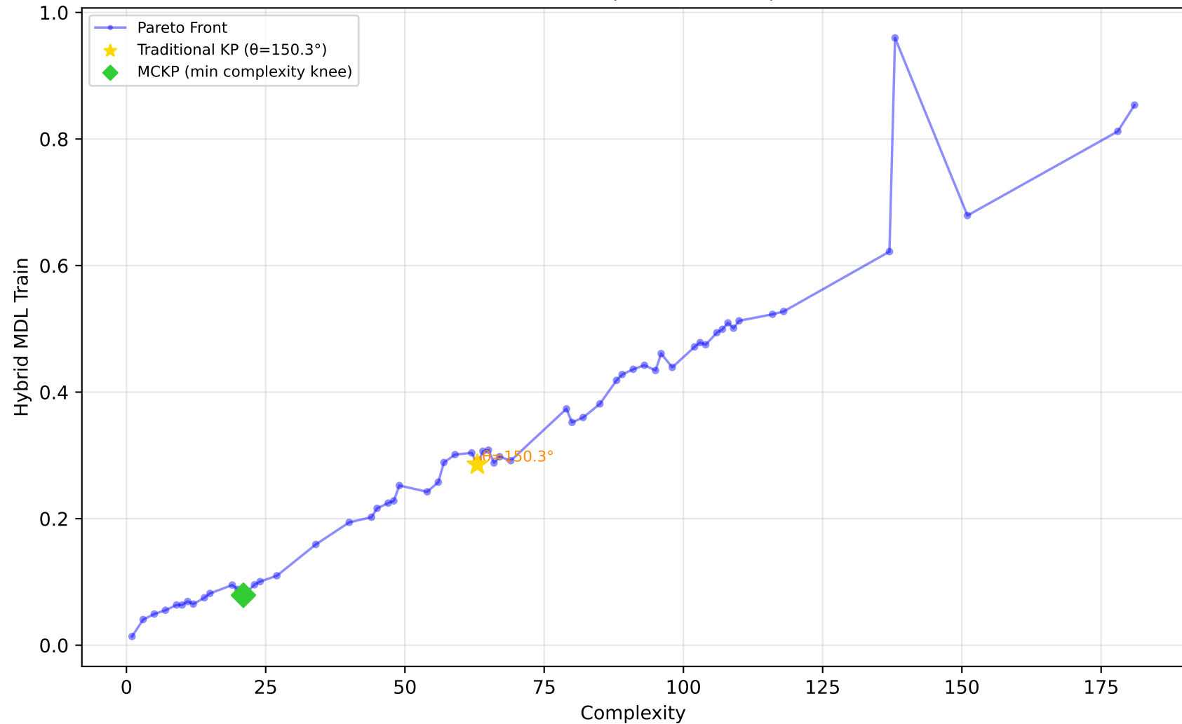
678_visualizing_environmental - Run 30 - SVP - Hybrid MDL Train \lambda_1=0.40 , \lambda_2=0.00 , \lambda_3=0.00 | Difficulty: 0.38 | Method: mckp
