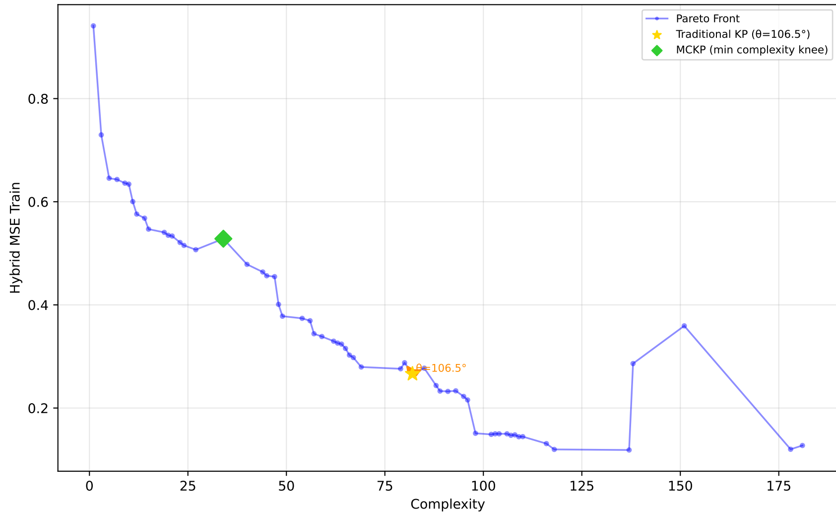
678_visualizing_environmental - Run 30 - SVP - Hybrid MSE Train \lambda_1=0.00, \lambda_2=0.10, \lambda_3=0.20 | Difficulty: 0.38 | Method: mckp
