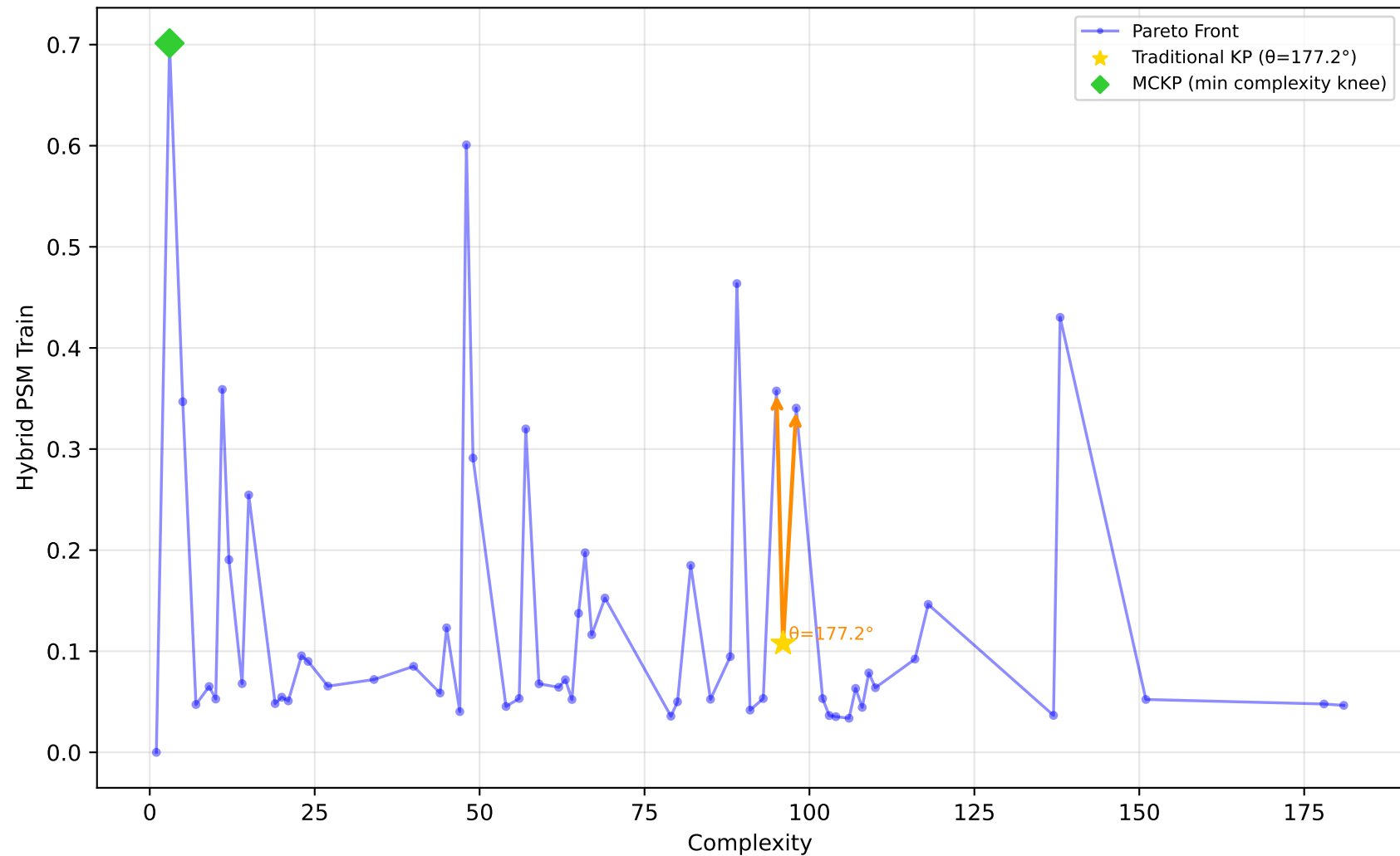
678_visualizing_environmental - Run 30 - SVP - Hybrid PSM Train \lambda_1=0.40, \lambda_2=0.00, \lambda_3=0.00 | Difficulty: 0.38 | Method: mckp
