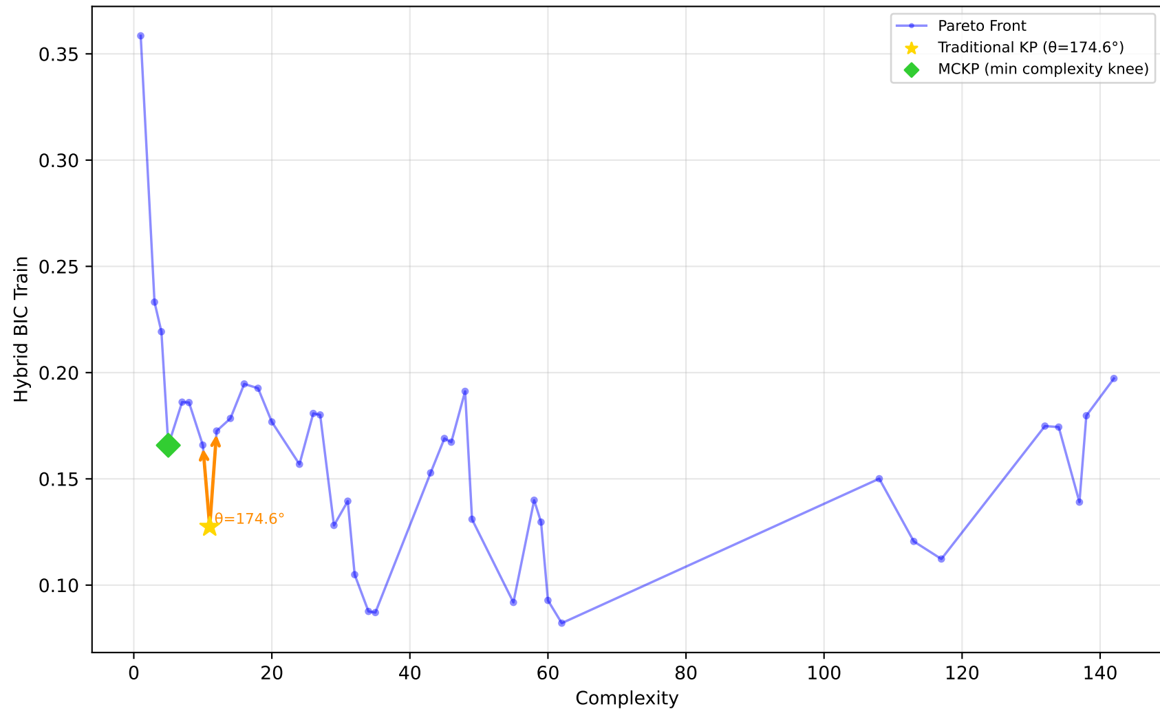
678_visualizing_environmental - Run 3 - MVP - Hybrid BIC Train \lambda_1=0.00, \lambda_2=0.00, \lambda_3=0.10 | Difficulty: 0.49 | Method: mckp
