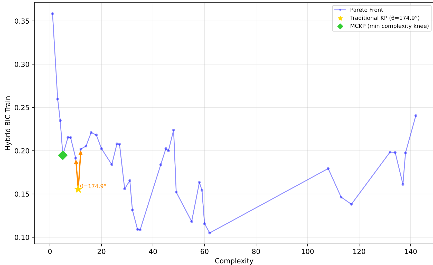
678_visualizing_environmental - Run 3 - MVP - Hybrid BIC Train \lambda_1=0.40, \lambda_2=0.00, \lambda_3=0.00 | Difficulty: 0.49 | Method: mckp
