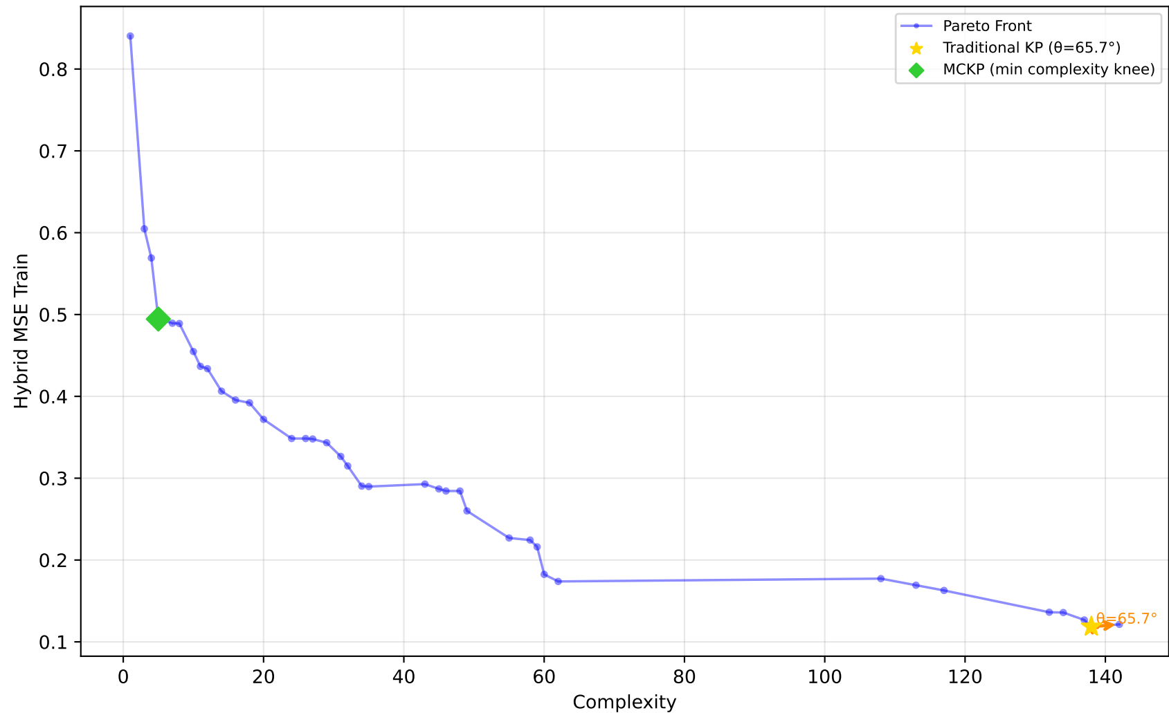
678_visualizing_environmental - Run 3 - MVP - Hybrid MSE Train \lambda_1=0.40, \lambda_2=0.00, \lambda_3=0.00 | Difficulty: 0.49 | Method: mckp
