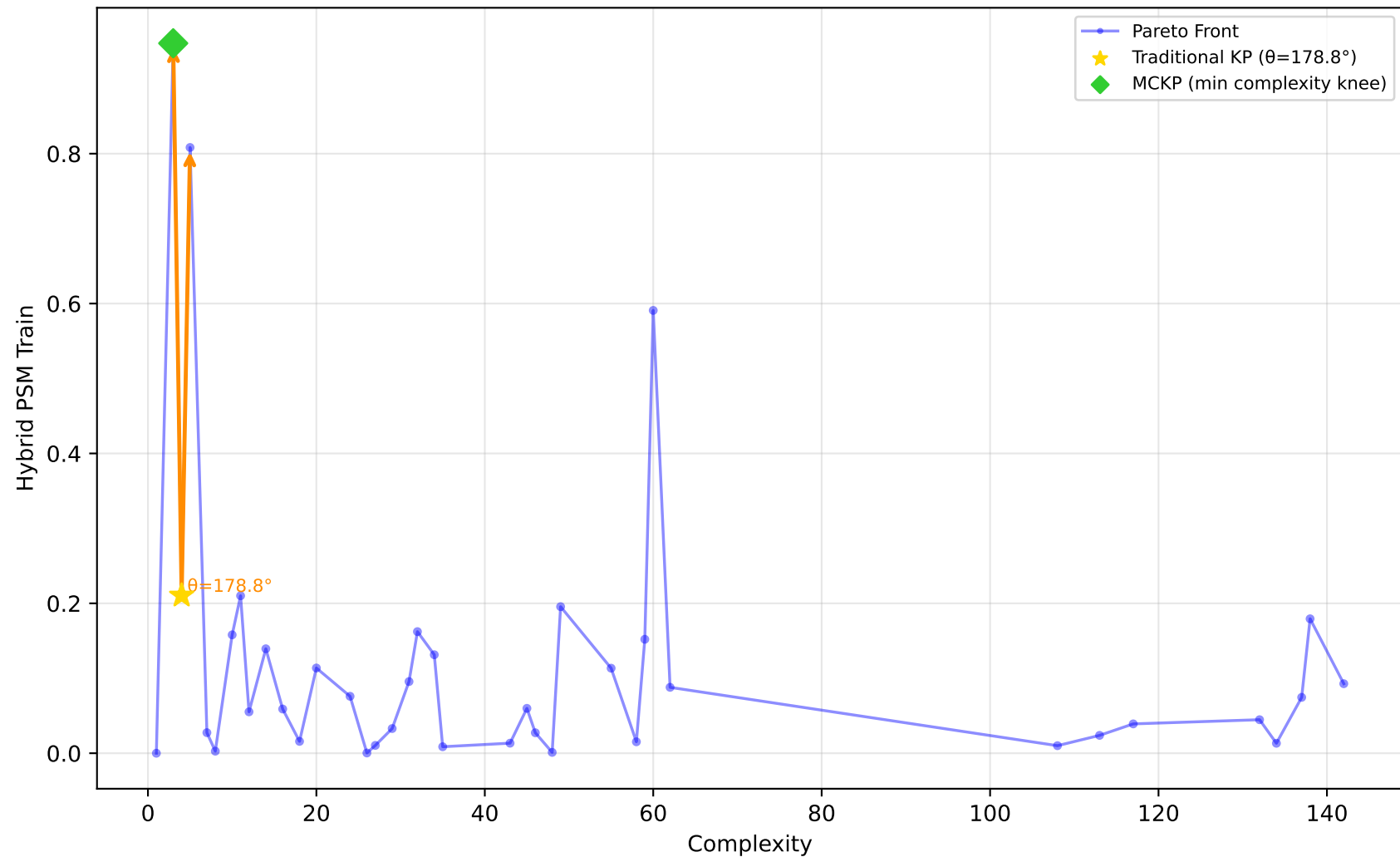
678_visualizing_environmental - Run 3 - MVP - Hybrid PSM Train \lambda_1=0.00, \lambda_2=0.00, \lambda_3=0.10 | Difficulty: 0.49 | Method: mckp
