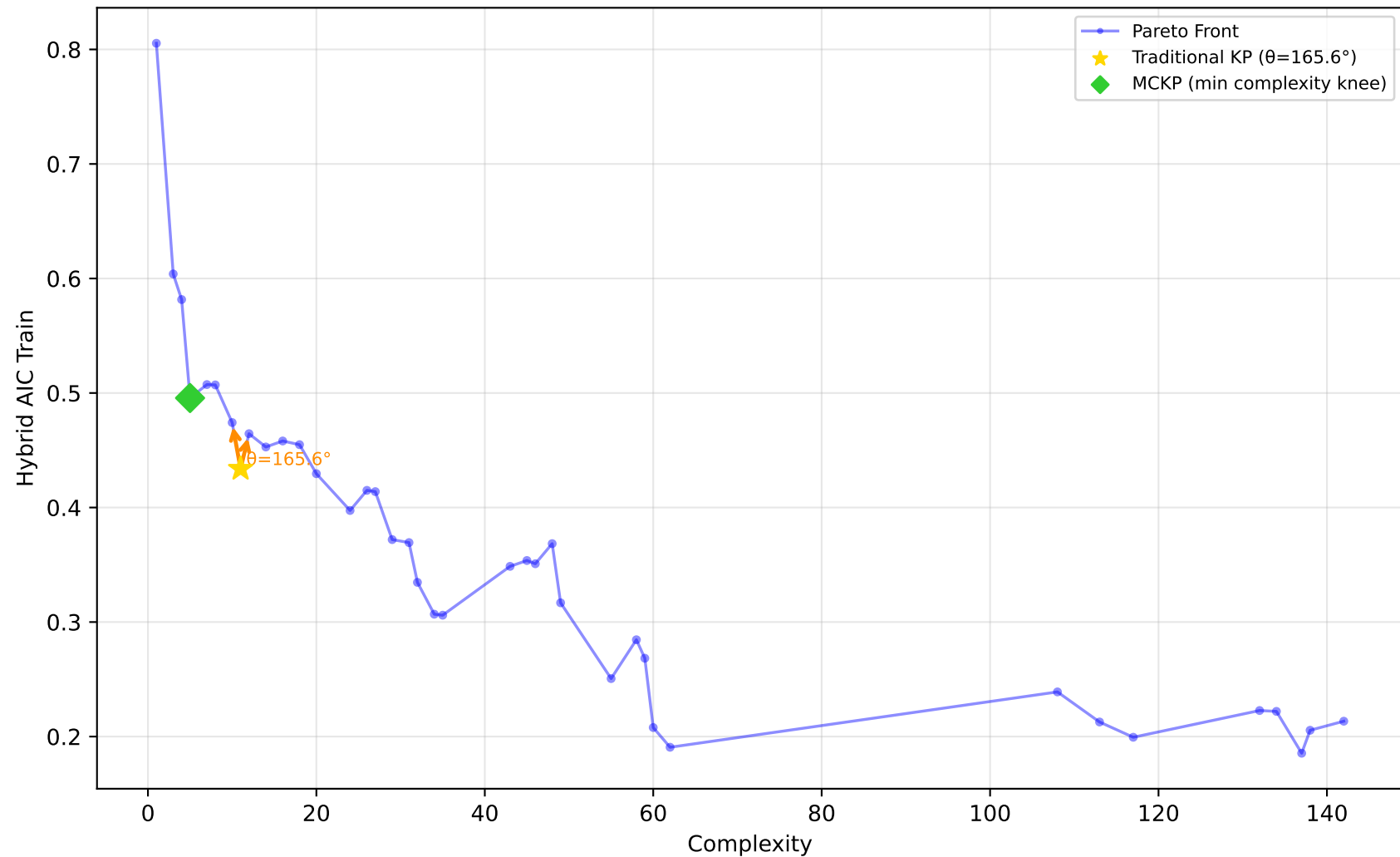
678_visualizing_environmental - Run 3 - SVP - Hybrid AIC Train \lambda_1=0.00, \lambda_2=0.10, \lambda_3=0.20 | Difficulty: 0.49 | Method: mckp
