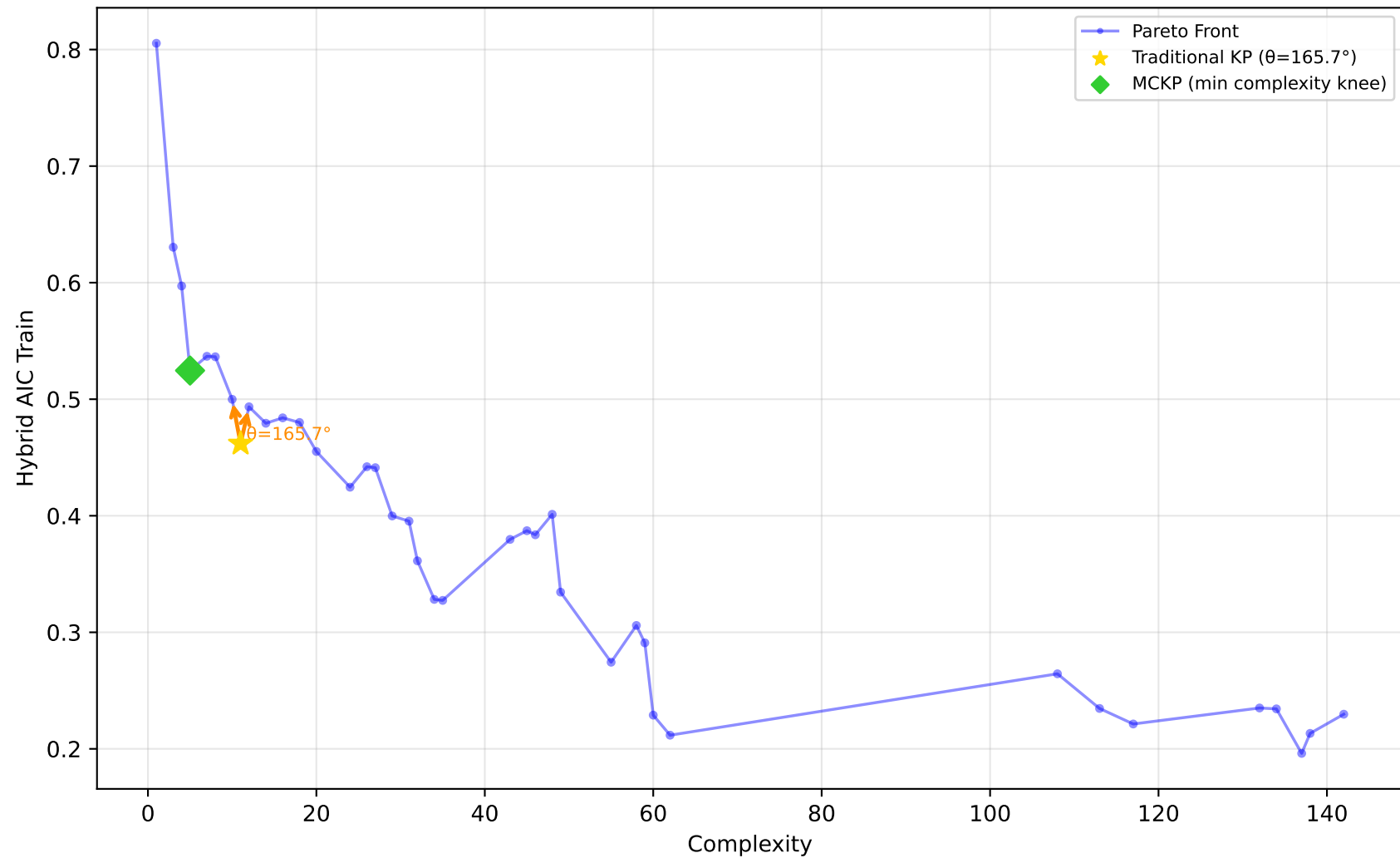
678_visualizing_environmental - Run 3 - SVP - Hybrid AIC Train \lambda_1=0.40, \lambda_2=0.00, \lambda_3=0.00 | Difficulty: 0.49 | Method: mckp
