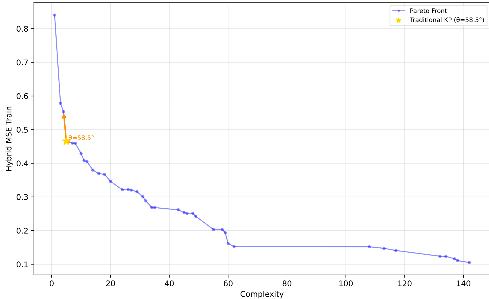
678_visualizing_environmental - Run 3 - SVP - Hybrid MSE Train \lambda_1=0.00, \lambda_2=0.10, \lambda_3=0.20 | Difficulty: 0.49 | Method: mckp
