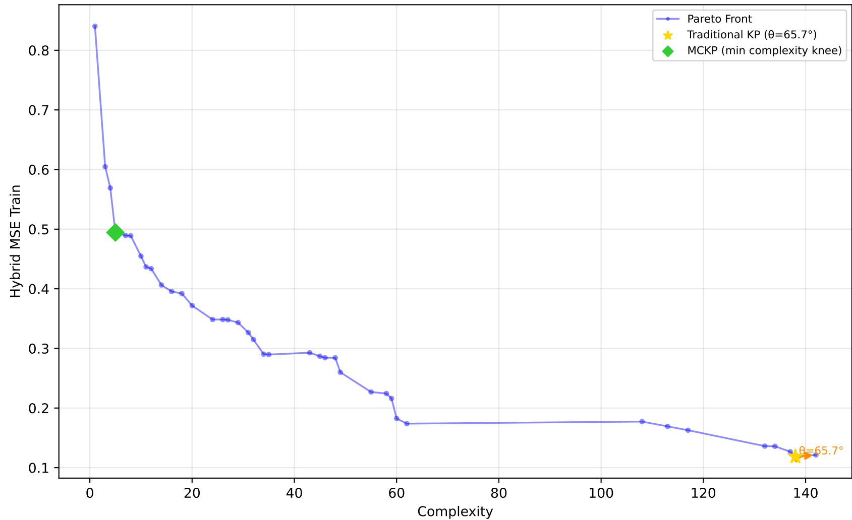
678_visualizing_environmental - Run 3 - SVP - Hybrid MSE Train \lambda_1=0.40, \lambda_2=0.00, \lambda_3=0.00 | Difficulty: 0.49 | Method: mckp
