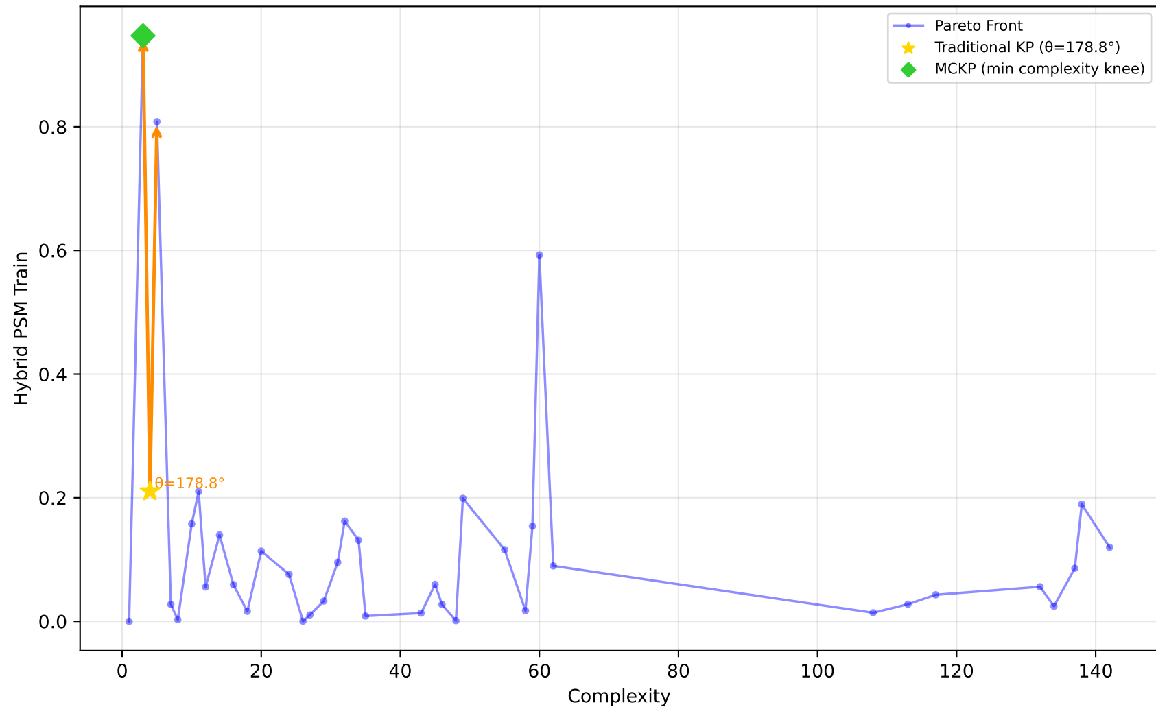
678_visualizing_environmental - Run 3 - SVP - Hybrid PSM Train \lambda_1=0.00, \lambda_2=0.10, \lambda_3=0.20 | Difficulty: 0.49 | Method: mckp
