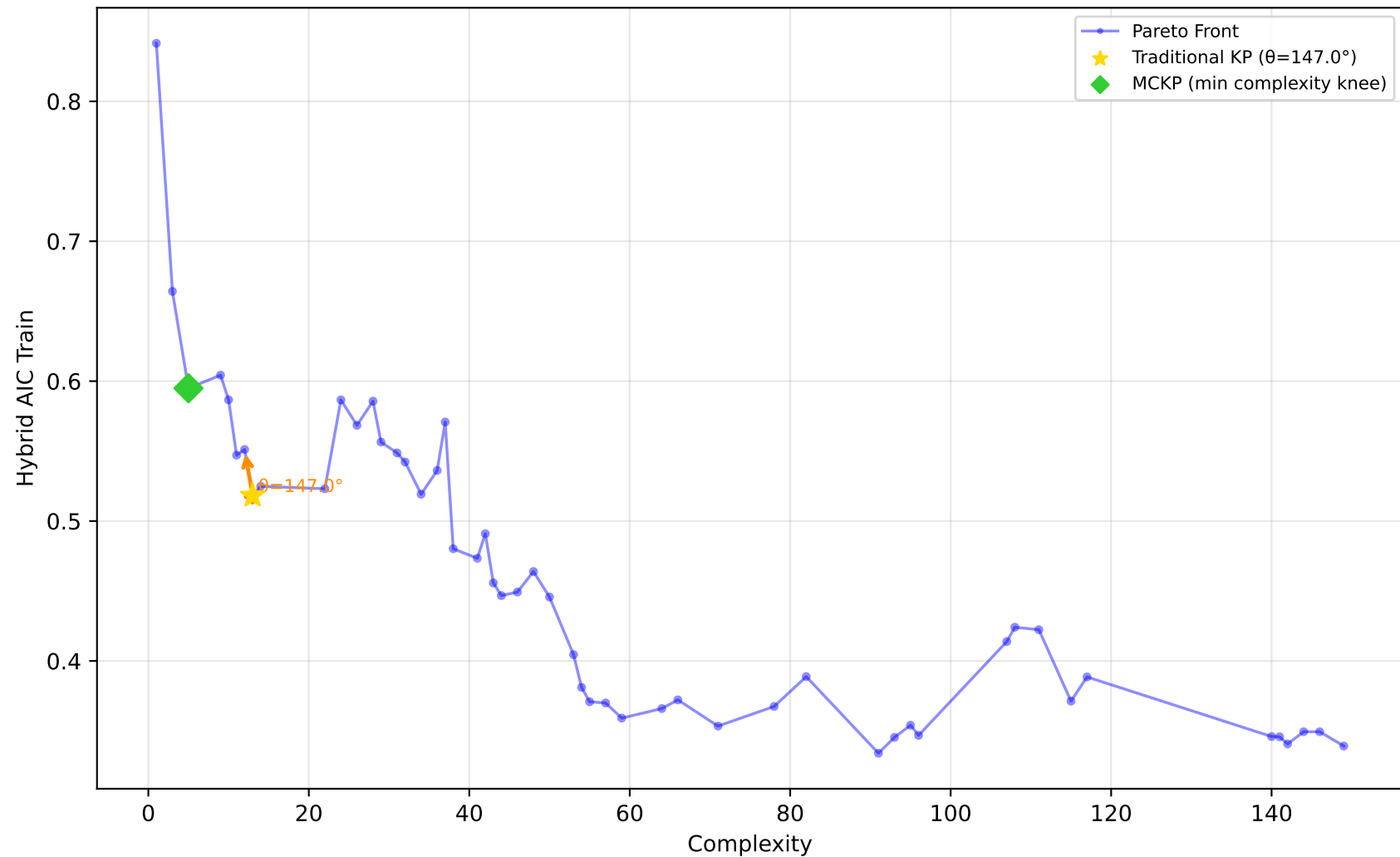
678_visualizing_environmental - Run 4 - MVP - Hybrid AIC Train \lambda_1=0.00 , \lambda_2=0.00 , \lambda_3=0.10 | Difficulty: 0.50 | Method: mckp
