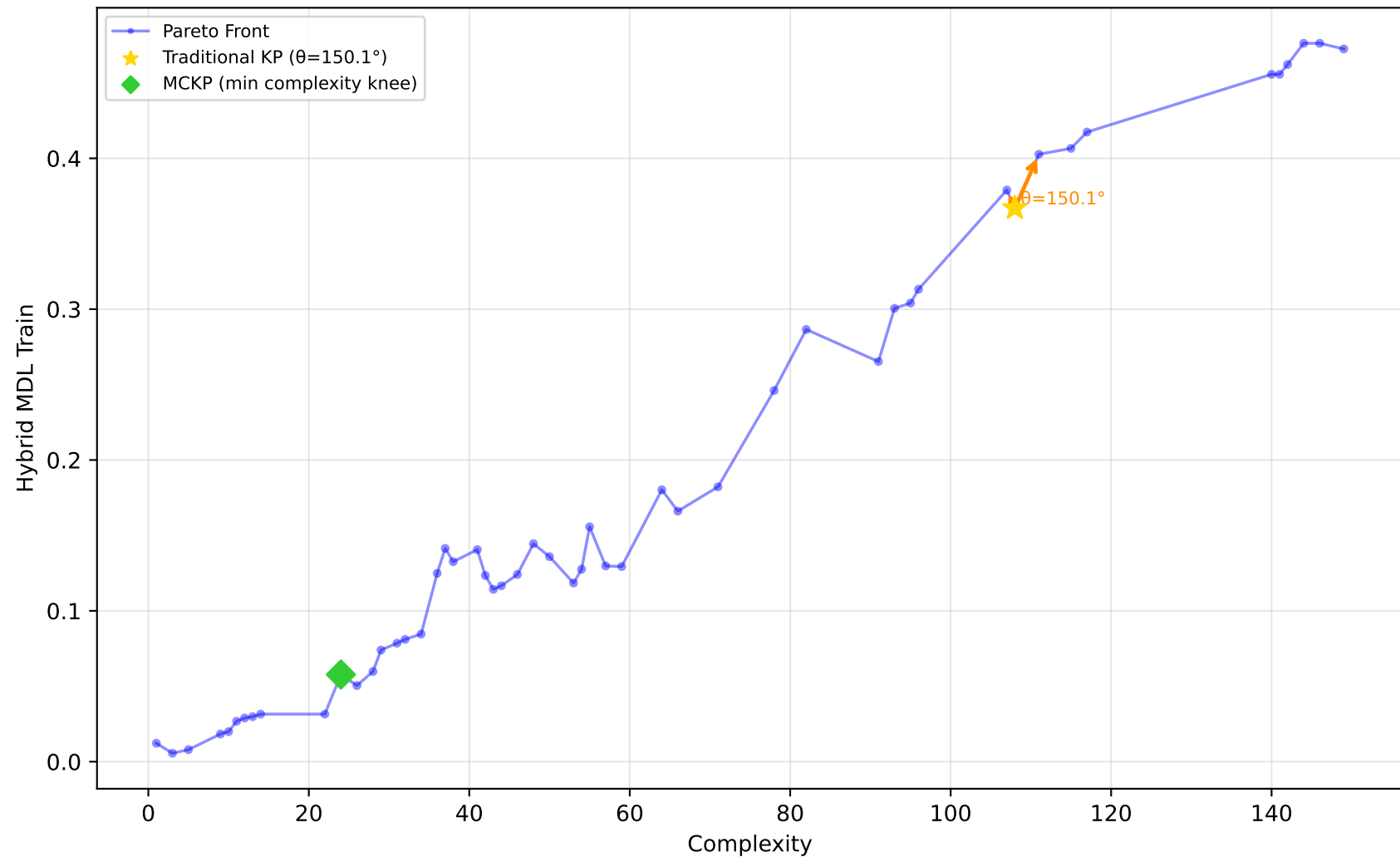
678_visualizing_environmental - Run 4 - MVP - Hybrid MDL Train \lambda_1=0.00, \lambda_2=0.00, \lambda_3=0.10 | Difficulty: 0.50 | Method: mckp
