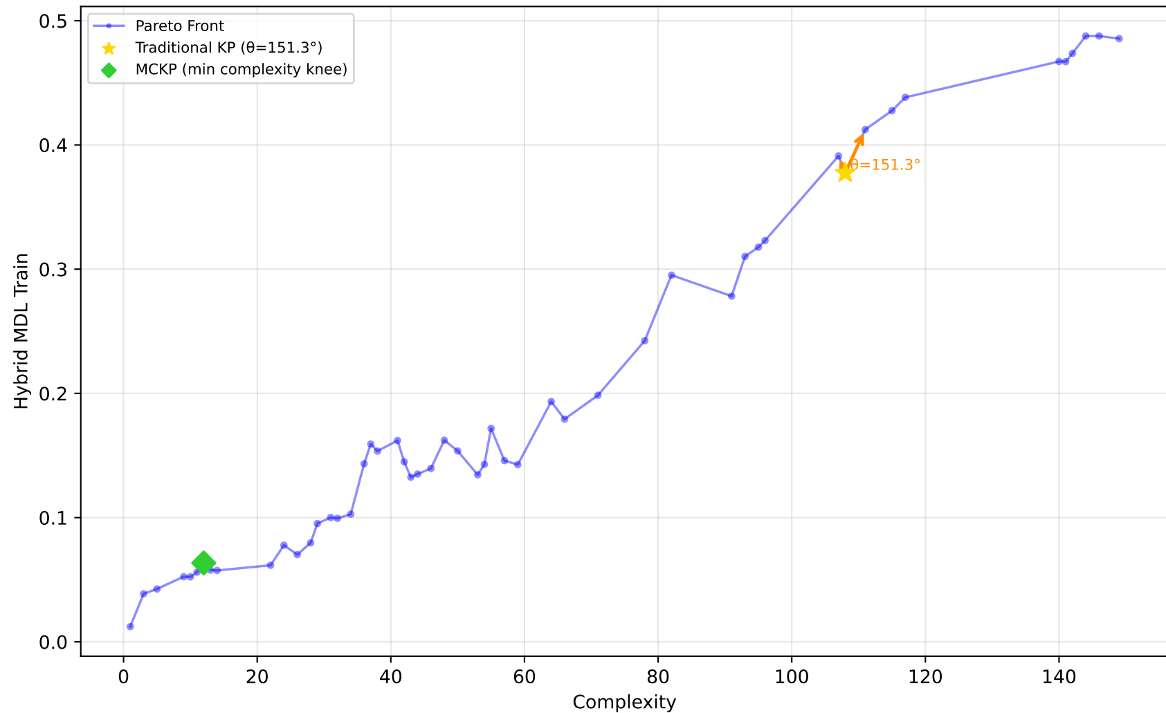
678_visualizing_environmental - Run 4 - MVP - Hybrid MDL Train \lambda_1=0.40, \lambda_2=0.00, \lambda_3=0.00 | Difficulty: 0.50 | Method: mckp
