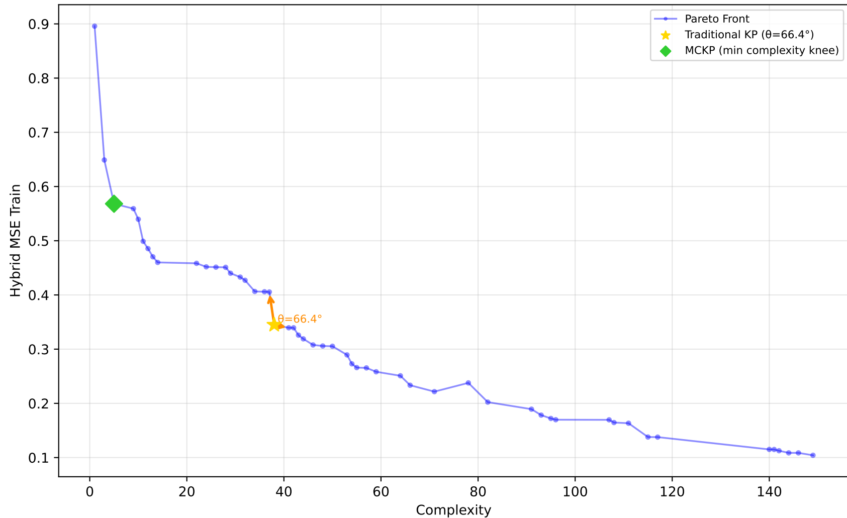
678_visualizing_environmental - Run 4 - MVP - Hybrid MSE Train \lambda_1=0.00, \lambda_2=0.00, \lambda_3=0.10 | Difficulty: 0.50 | Method: mckp
