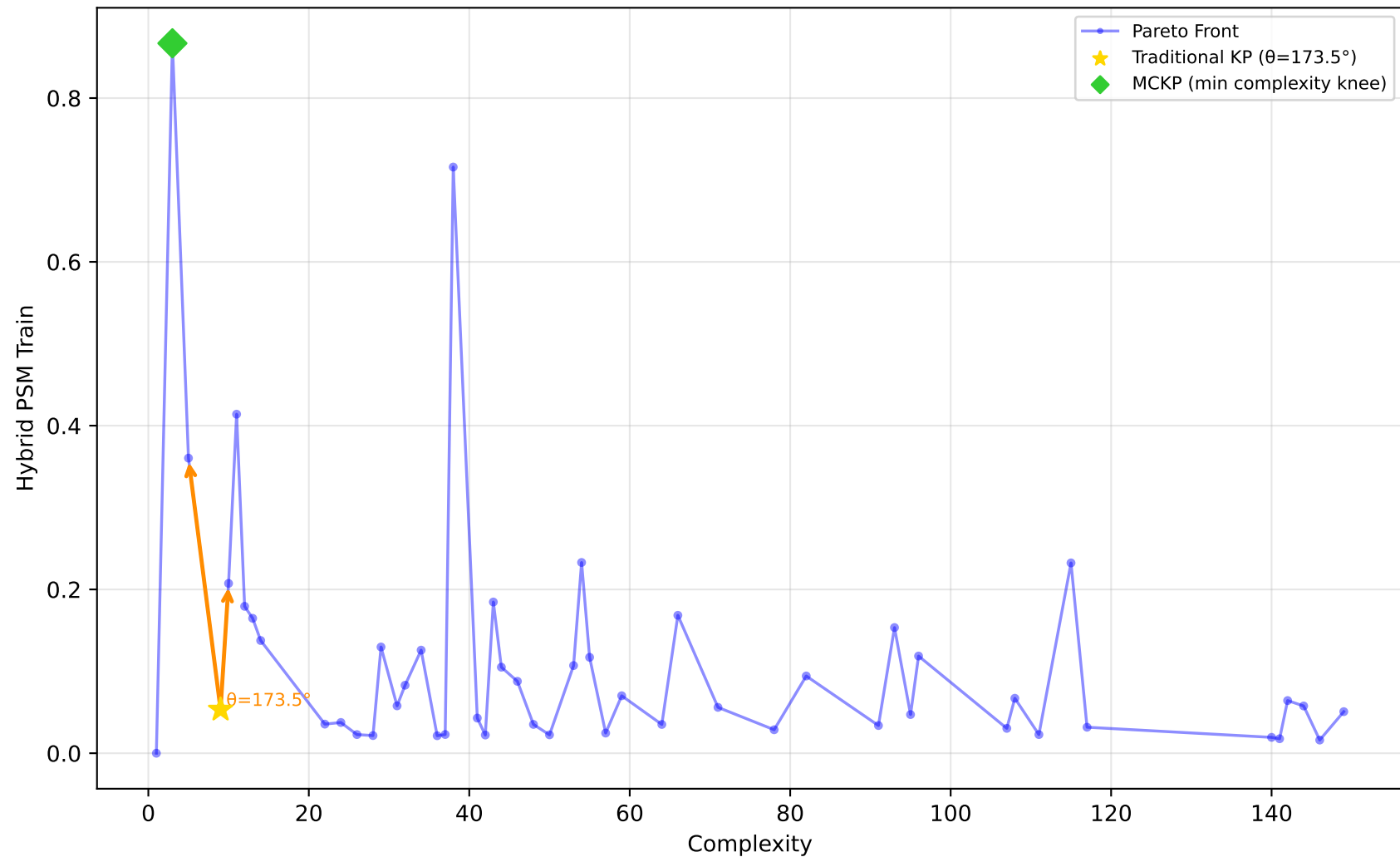
678_visualizing_environmental - Run 4 - MVP - Hybrid PSM Train \lambda_1=0.40, \lambda_2=0.00, \lambda_3=0.00 | Difficulty: 0.50 | Method: mckp
