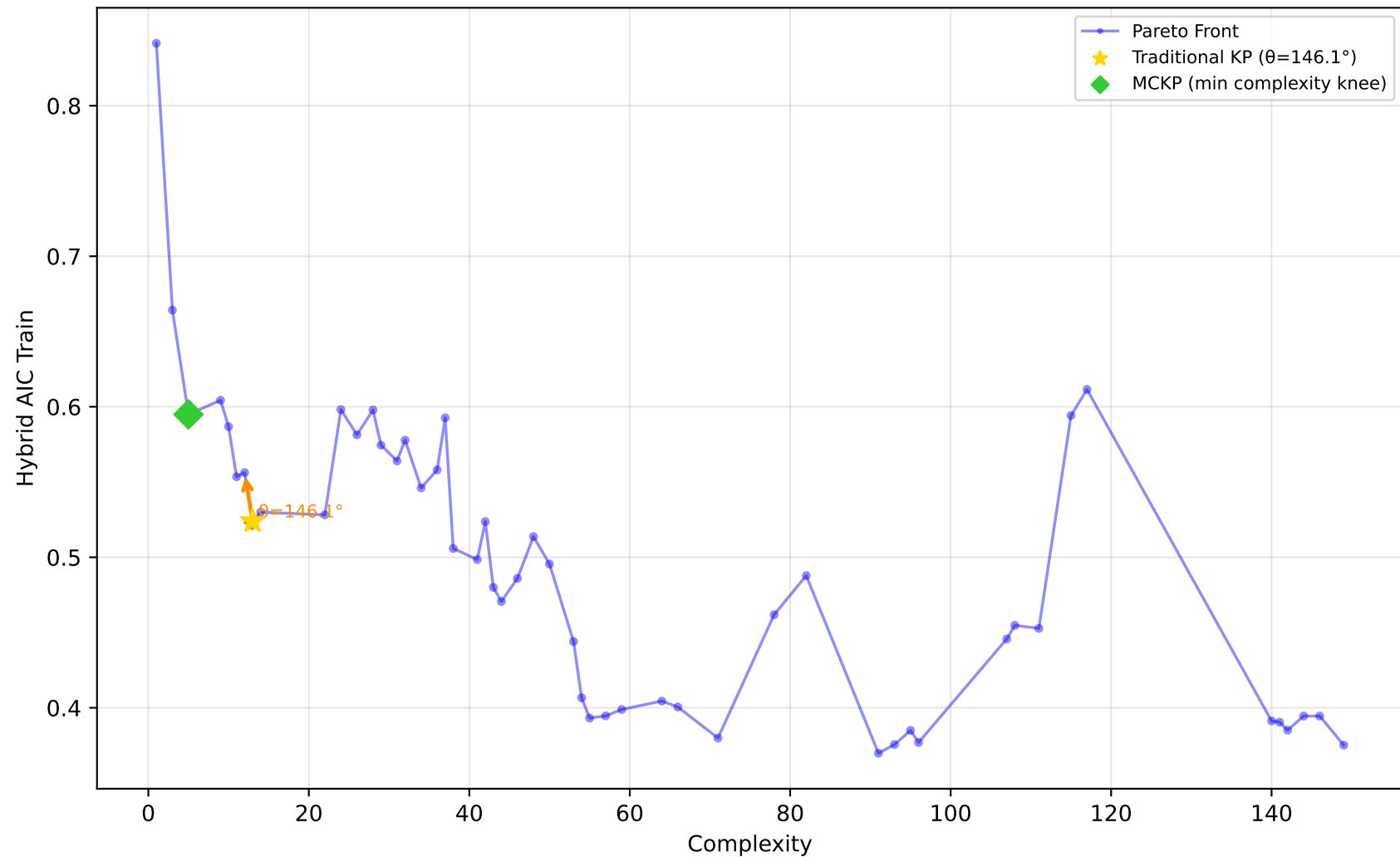
678_visualizing_environmental - Run 4 - SVP - Hybrid AIC Train \lambda_1=0.00, \lambda_2=0.10, \lambda_3=0.20 | Difficulty: 0.50 | Method: mckp
