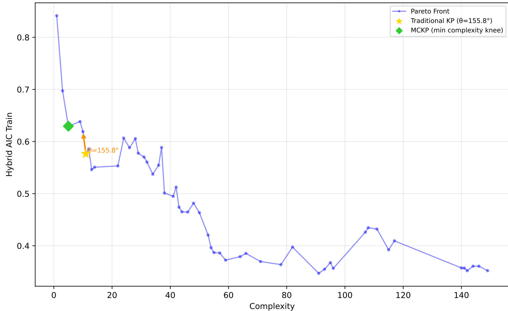
678_visualizing_environmental - Run 4 - SVP - Hybrid AIC Train \lambda_1=0.40, \lambda_2=0.00, \lambda_3=0.00 | Difficulty: 0.50 | Method: mckp
