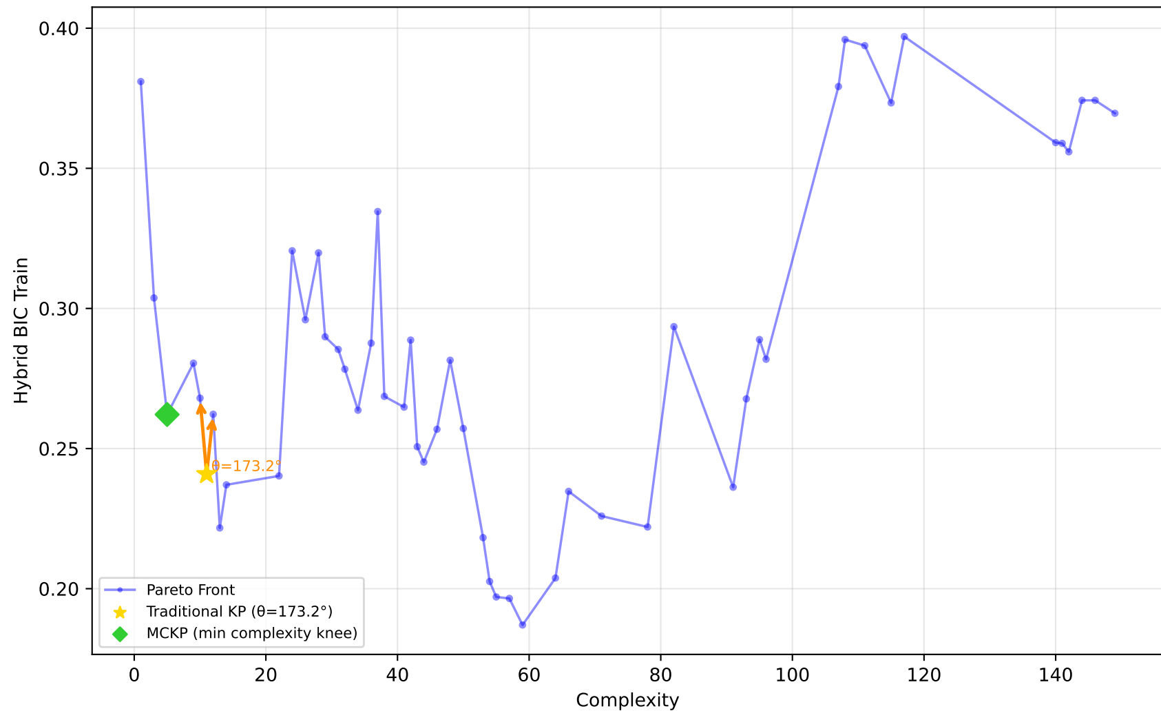
678_visualizing_environmental - Run 4 - SVP - Hybrid BIC Train \lambda_1=0.40 , \lambda_2=0.00 , \lambda_3=0.00 | Difficulty: 0.50 | Method: mckp
