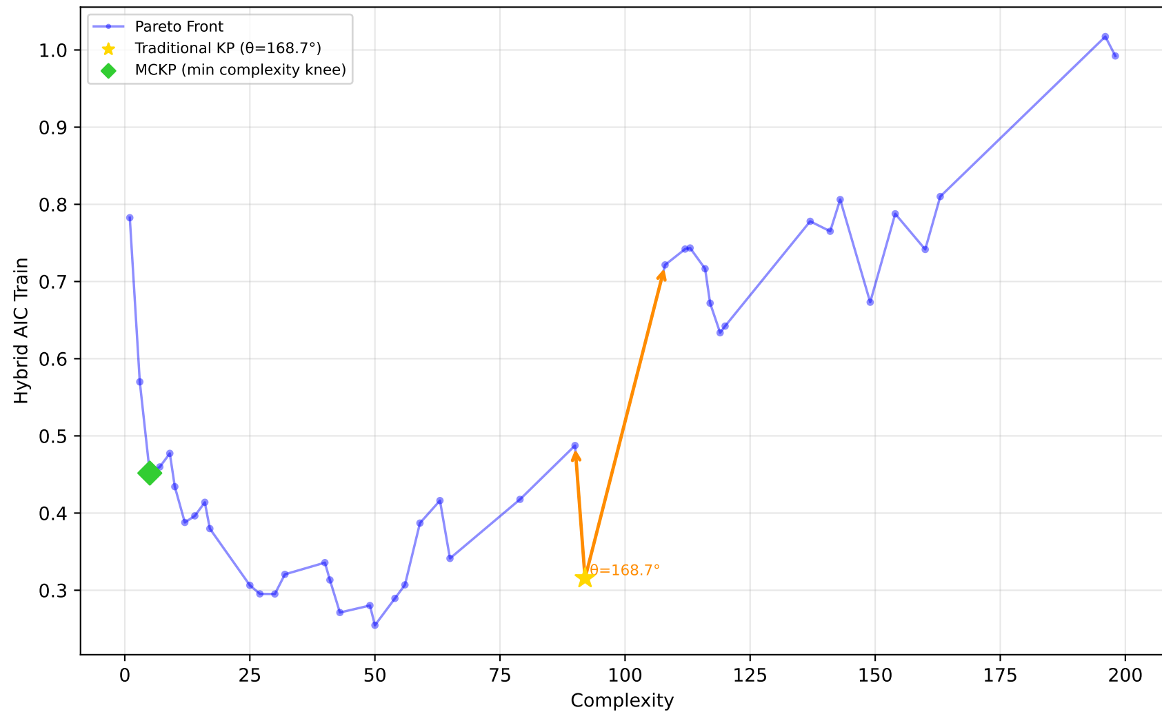
678_visualizing_environmental - Run 5 - MVP - Hybrid AIC Train \lambda_1=0.00, \lambda_2=0.00, \lambda_3=0.10 | Difficulty: 0.12 | Method: mckp
