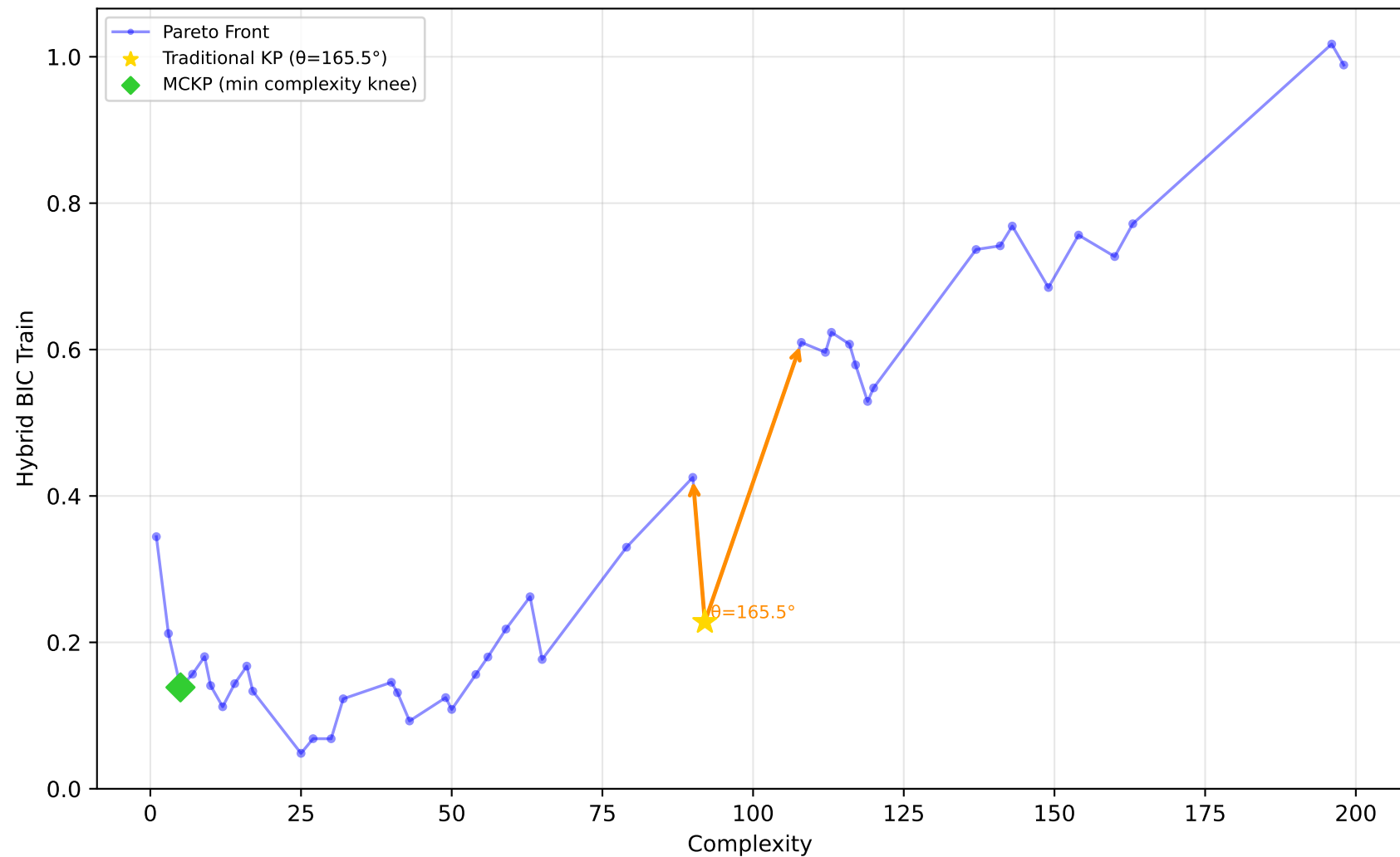
678_visualizing_environmental - Run 5 - MVP - Hybrid BIC Train \lambda_1=0.00, \lambda_2=0.00, \lambda_3=0.10 | Difficulty: 0.12 | Method: mckp
