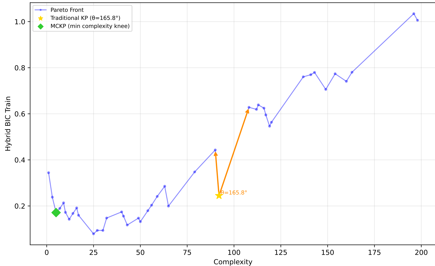
678_visualizing_environmental - Run 5 - MVP - Hybrid BIC Train \lambda_1=0.40, \lambda_2=0.00, \lambda_3=0.00 | Difficulty: 0.12 | Method: mckp
