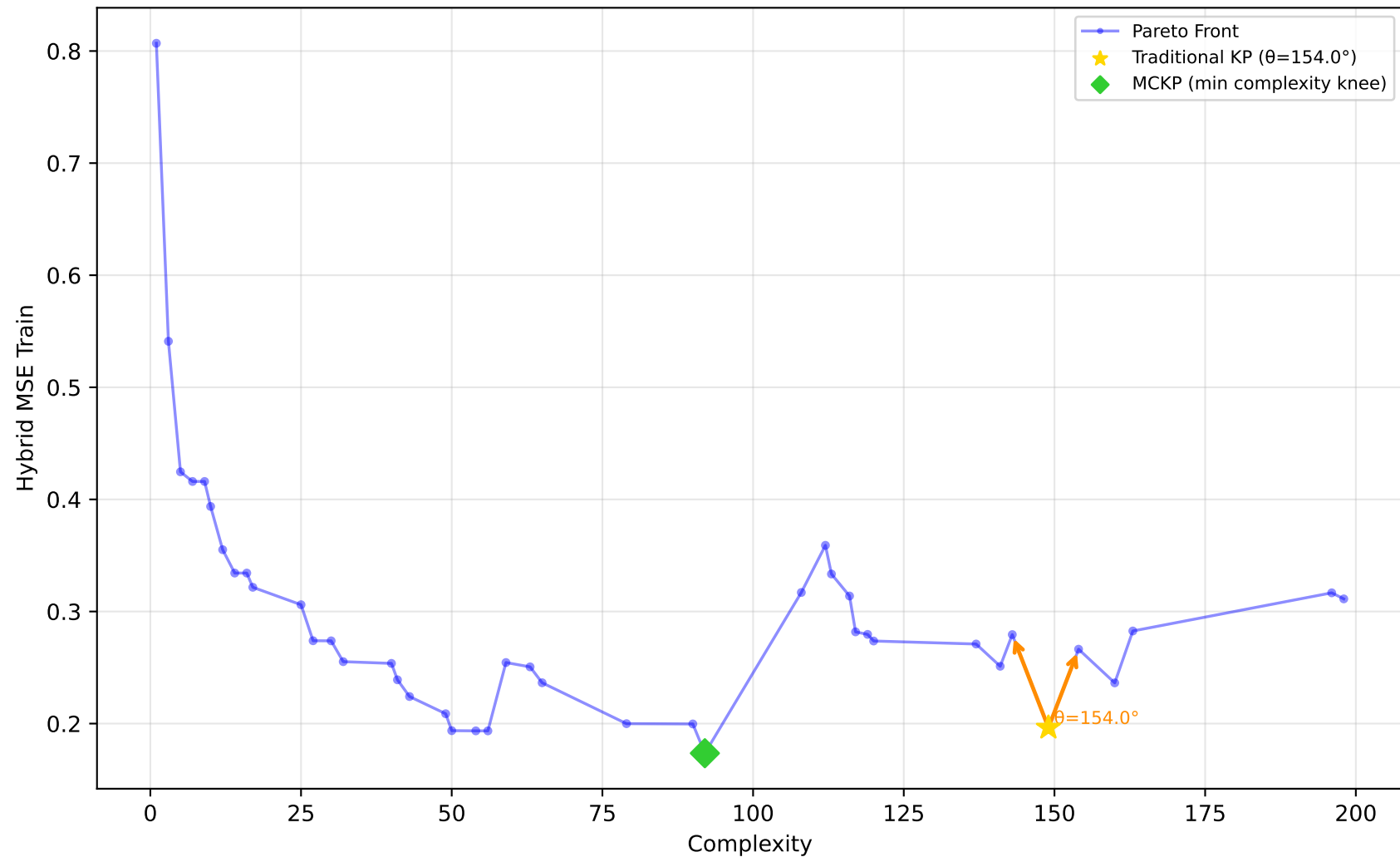
678_visualizing_environmental - Run 5 - MVP - Hybrid MSE Train \lambda_1=0.00, \lambda_2=0.00, \lambda_3=0.10 | Difficulty: 0.12 | Method: mckp
