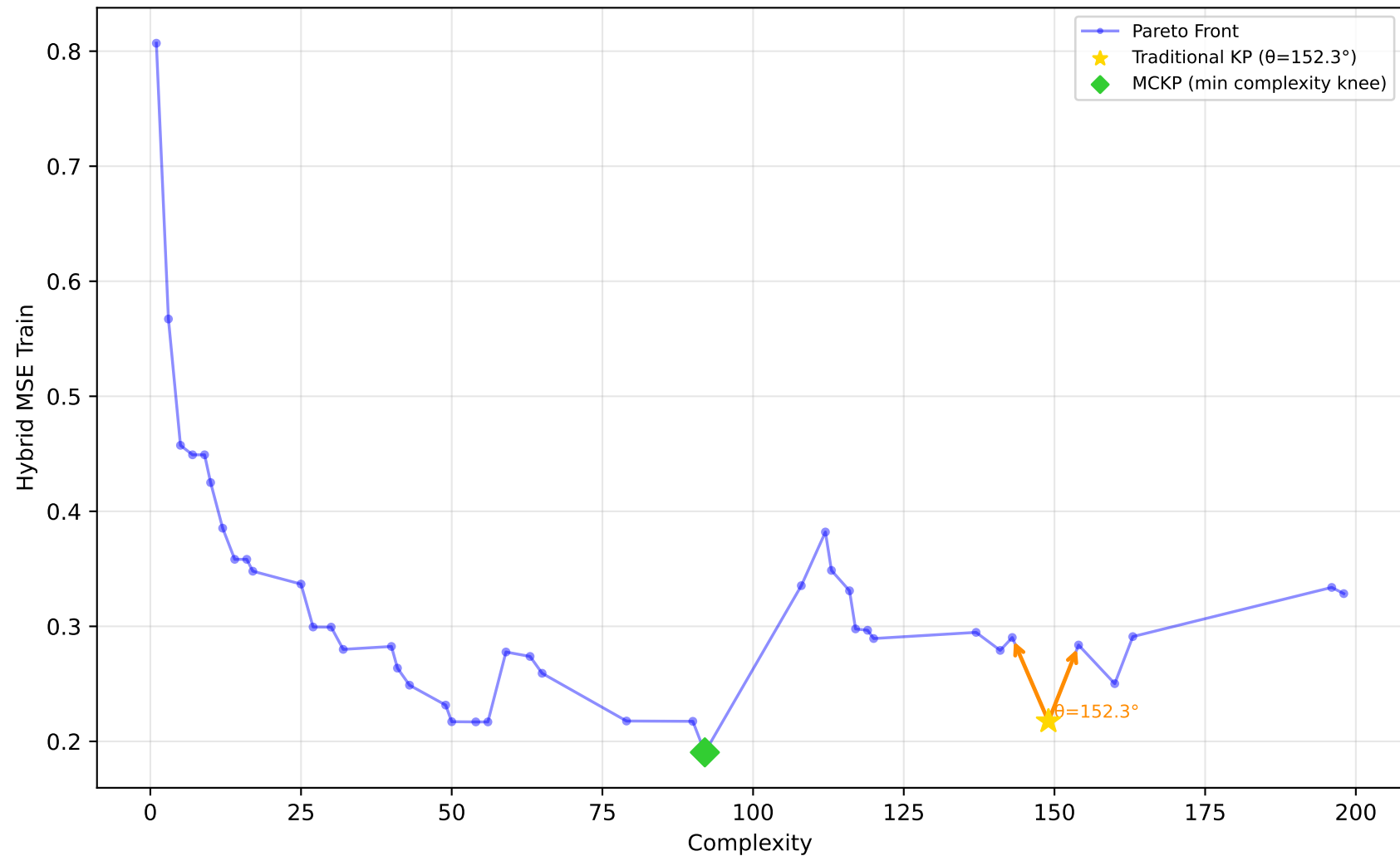
678_visualizing_environmental - Run 5 - MVP - Hybrid MSE Train \lambda_1=0.40, \lambda_2=0.00, \lambda_3=0.00 | Difficulty: 0.12 | Method: mckp
