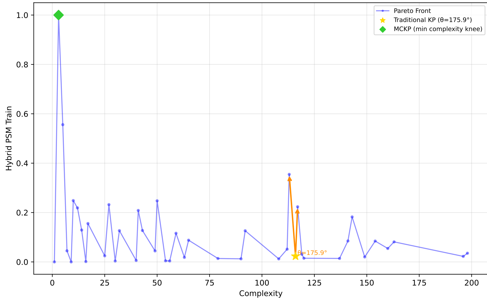
678_visualizing_environmental - Run 5 - MVP - Hybrid PSM Train \lambda_1=0.00, \lambda_2=0.00, \lambda_3=0.10 | Difficulty: 0.12 | Method: mckp
