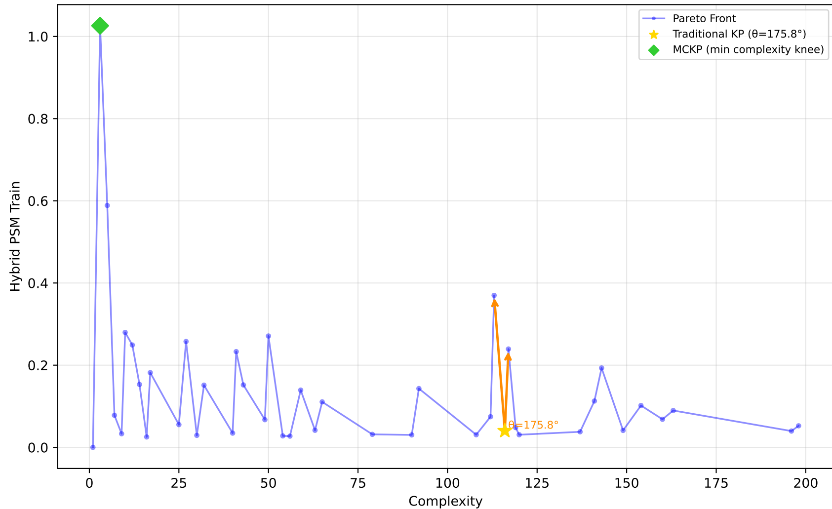
678_visualizing_environmental - Run 5 - MVP - Hybrid PSM Train \lambda_1=0.40, \lambda_2=0.00, \lambda_3=0.00 | Difficulty: 0.12 | Method: mckp
