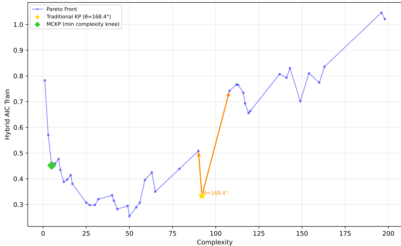
678_visualizing_environmental - Run 5 - SVP - Hybrid AIC Train \lambda_1=0.00 , \lambda_2=0.10 , \lambda_3=0.20 | Difficulty: 0.12 | Method: mckp
