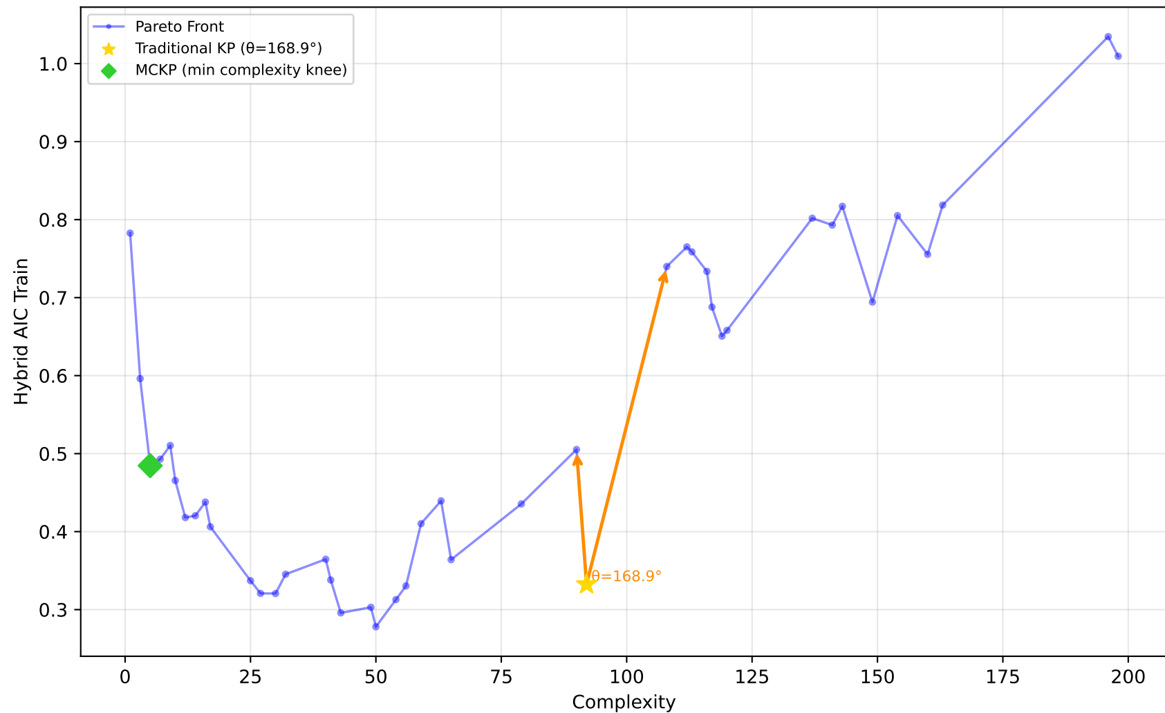
678_visualizing_environmental - Run 5 - SVP - Hybrid AIC Train \lambda_1=0.40 , \lambda_2=0.00 , \lambda_3=0.00 | Difficulty: 0.12 | Method: mckp
