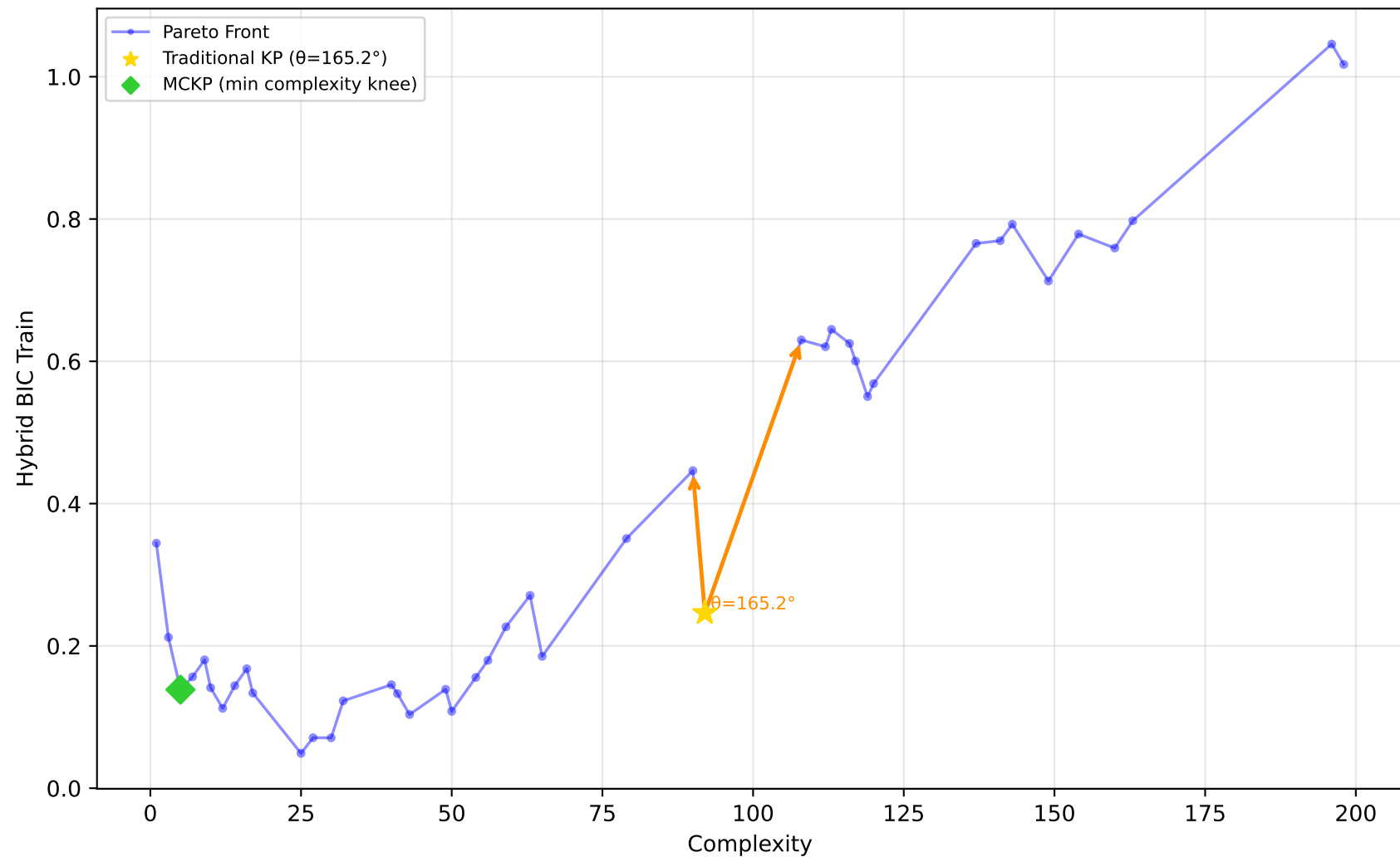
678_visualizing_environmental - Run 5 - SVP - Hybrid BIC Train \lambda_1=0.00, \lambda_2=0.10, \lambda_3=0.20 | Difficulty: 0.12 | Method: mckp
