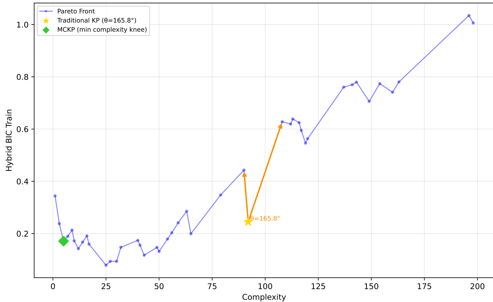
678_visualizing_environmental - Run 5 - SVP - Hybrid BIC Train \lambda_1=0.40 , \lambda_2=0.00 , \lambda_3=0.00 | Difficulty: 0.12 | Method: mckp
