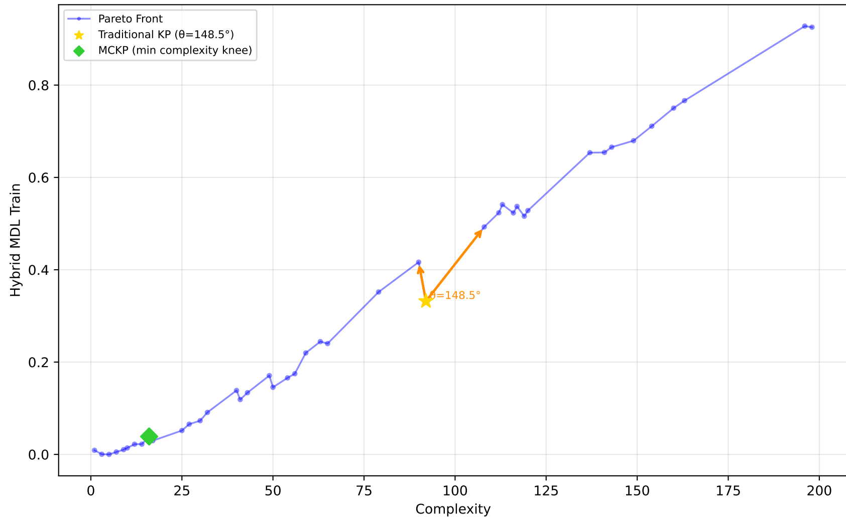
678_visualizing_environmental - Run 5 - SVP - Hybrid MDL Train \lambda_1=0.00, \lambda_2=0.10, \lambda_3=0.20 | Difficulty: 0.12 | Method: mckp
