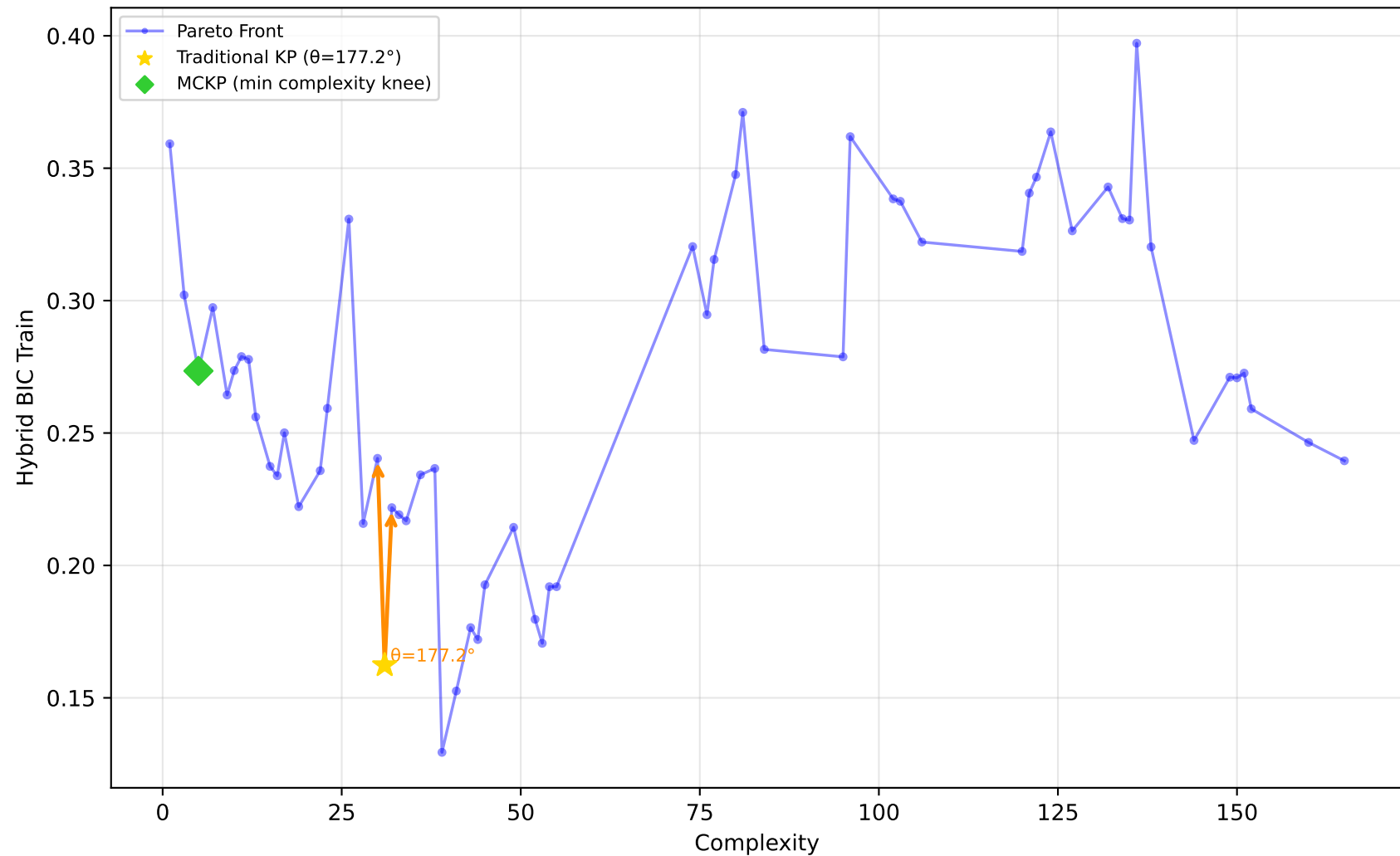
678_visualizing_environmental - Run 6 - MVP - Hybrid BIC Train \lambda_1=0.40, \lambda_2=0.00, \lambda_3=0.00 | Difficulty: 0.72 | Method: hmr
