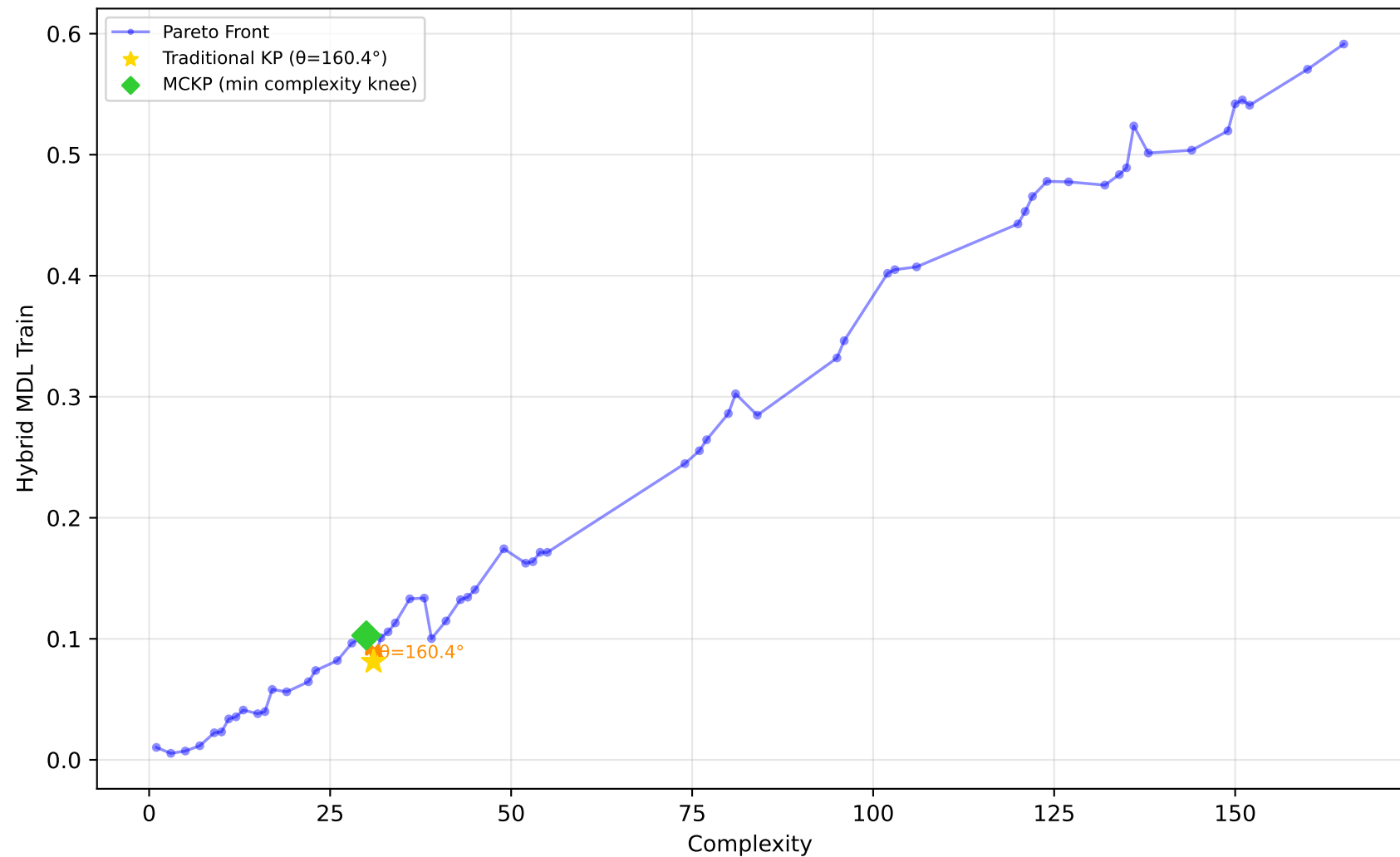
678_visualizing_environmental - Run 6 - MVP - Hybrid MDL Train \lambda_1=0.00, \lambda_2=0.00, \lambda_3=0.10 | Difficulty: 0.72 | Method: hmr
