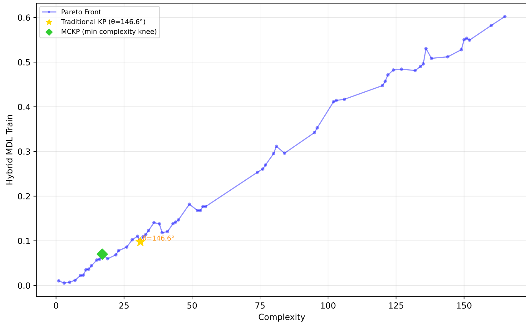
678_visualizing_environmental - Run 6 - SVP - Hybrid MDL Train \lambda_1=0.00, \lambda_2=0.10, \lambda_3=0.20 | Difficulty: 0.72 | Method: hmr
